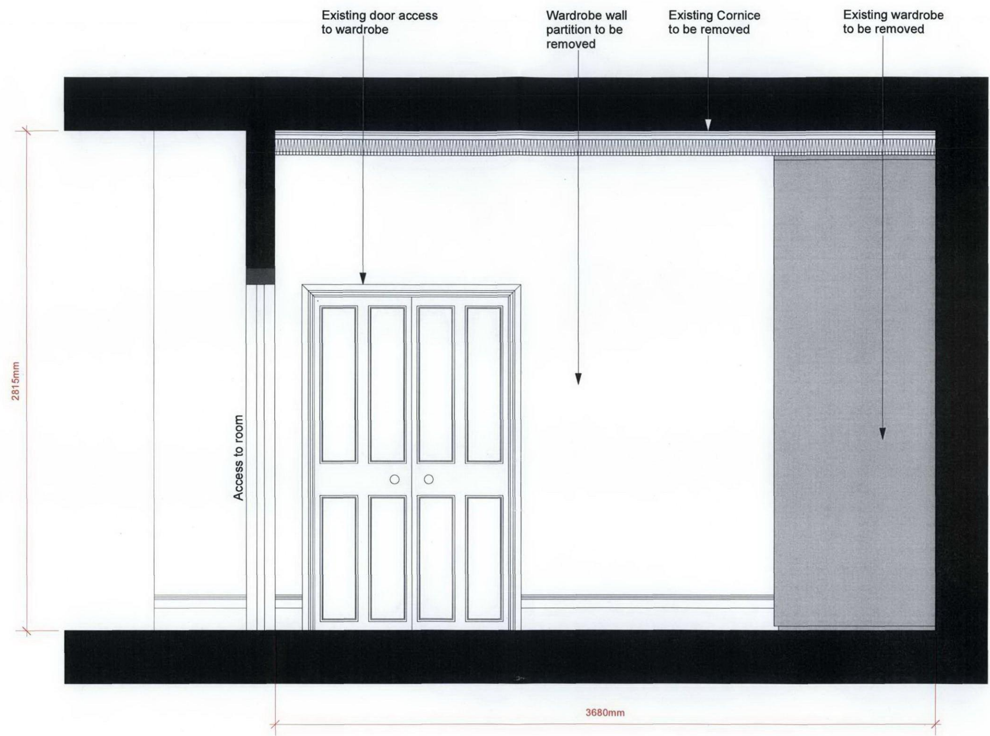
Elevation 1 - Dressing Room
