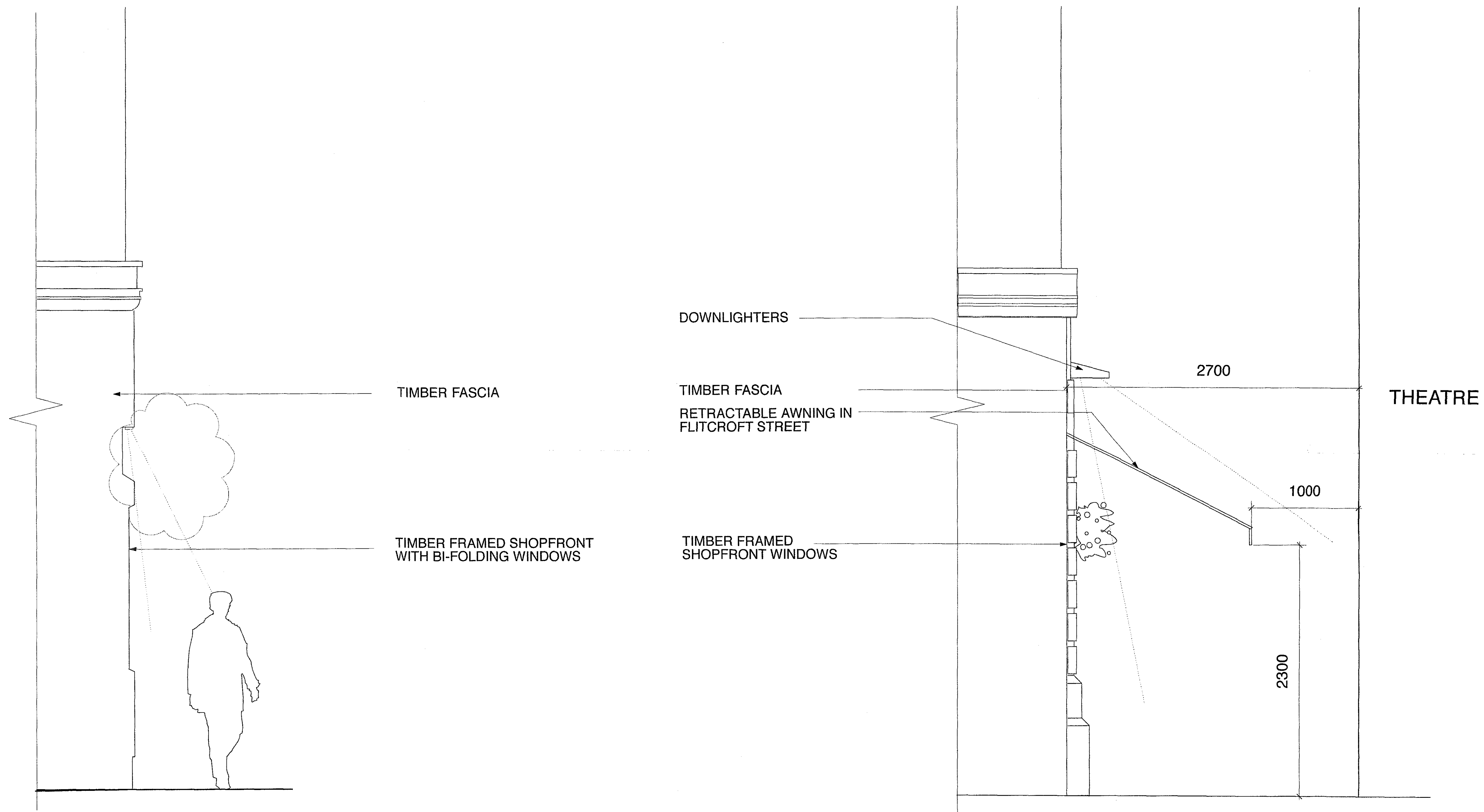
PROPOSED SHOPFRONT SECTION AA CHARING CROSS ROAD
