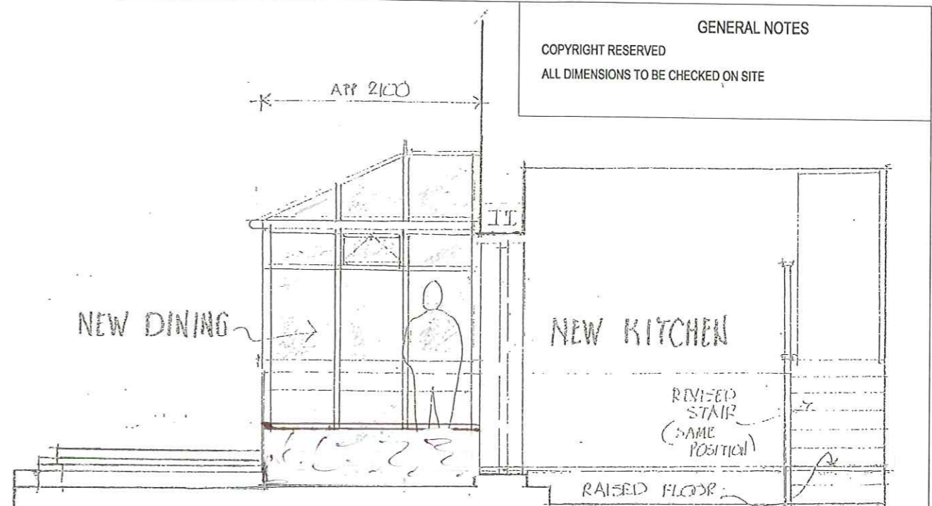
SECTION A-A PROPOSED
