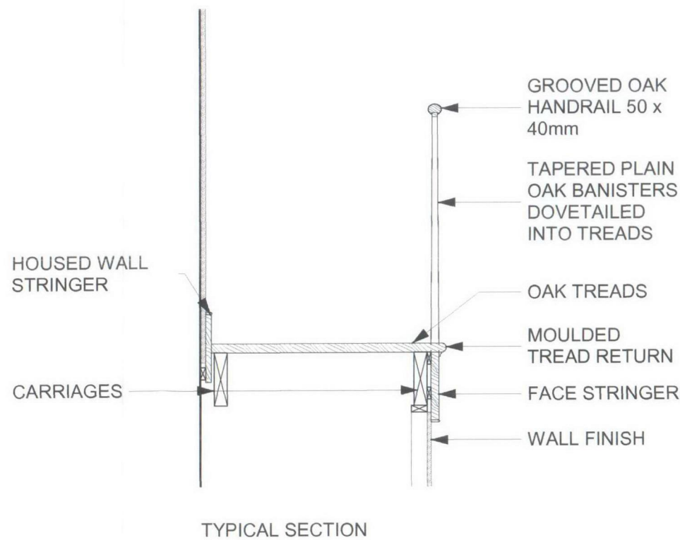
TYPICAL SECTION
