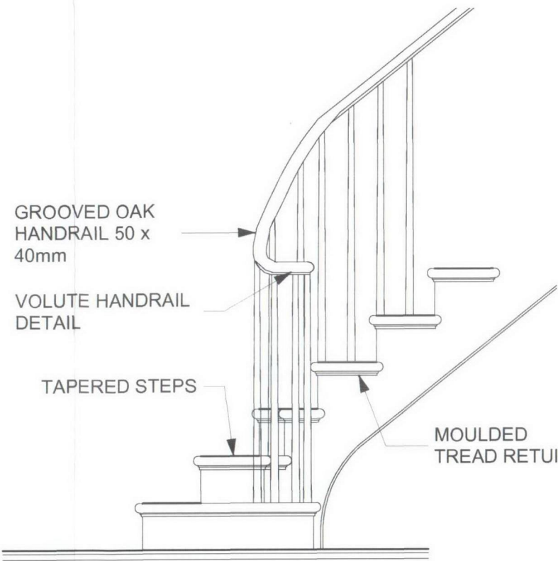
ELEVATION X AT GF LEVEL
