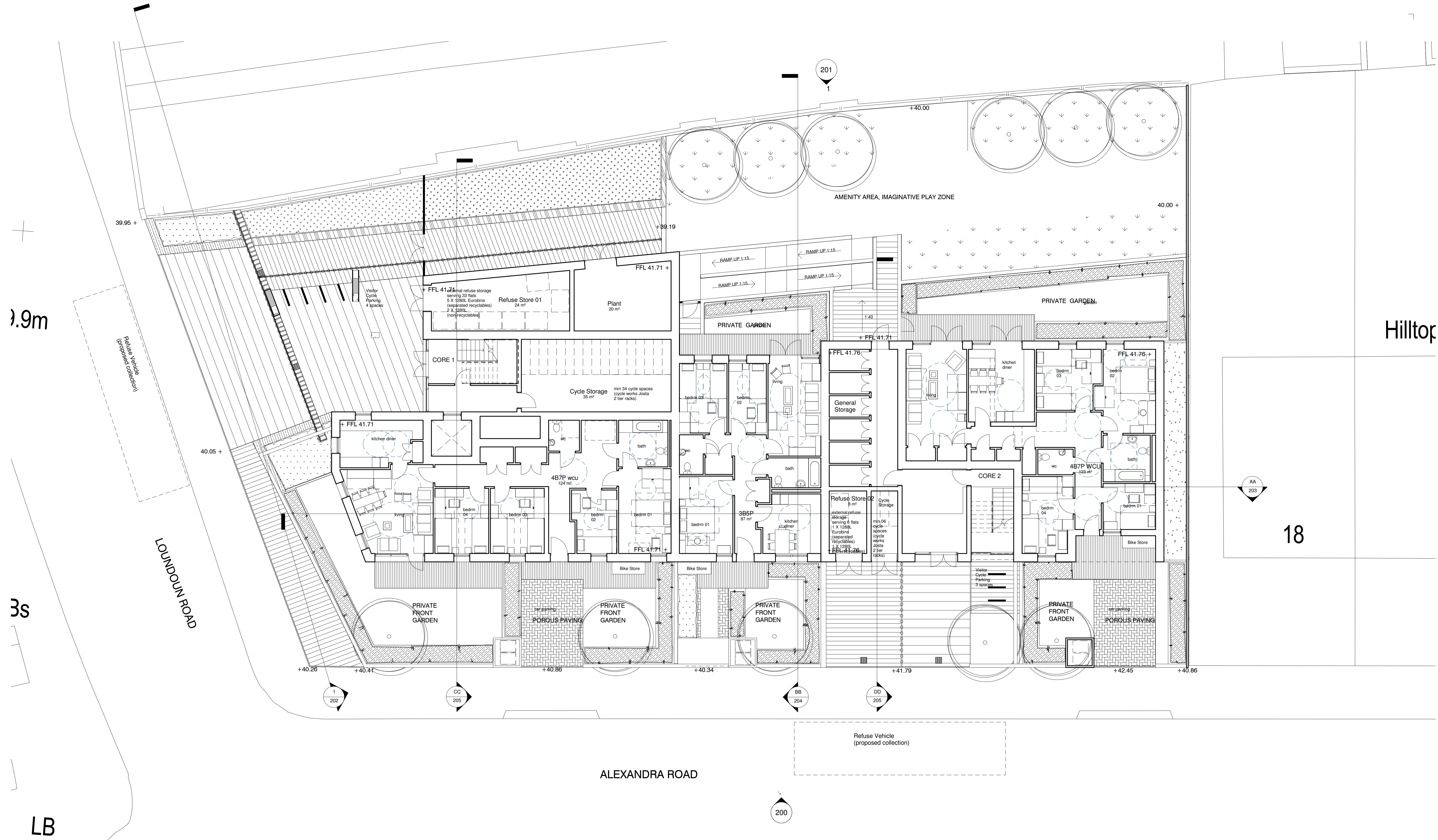
1 101 Ground Floor GA Plan 1 : 100
