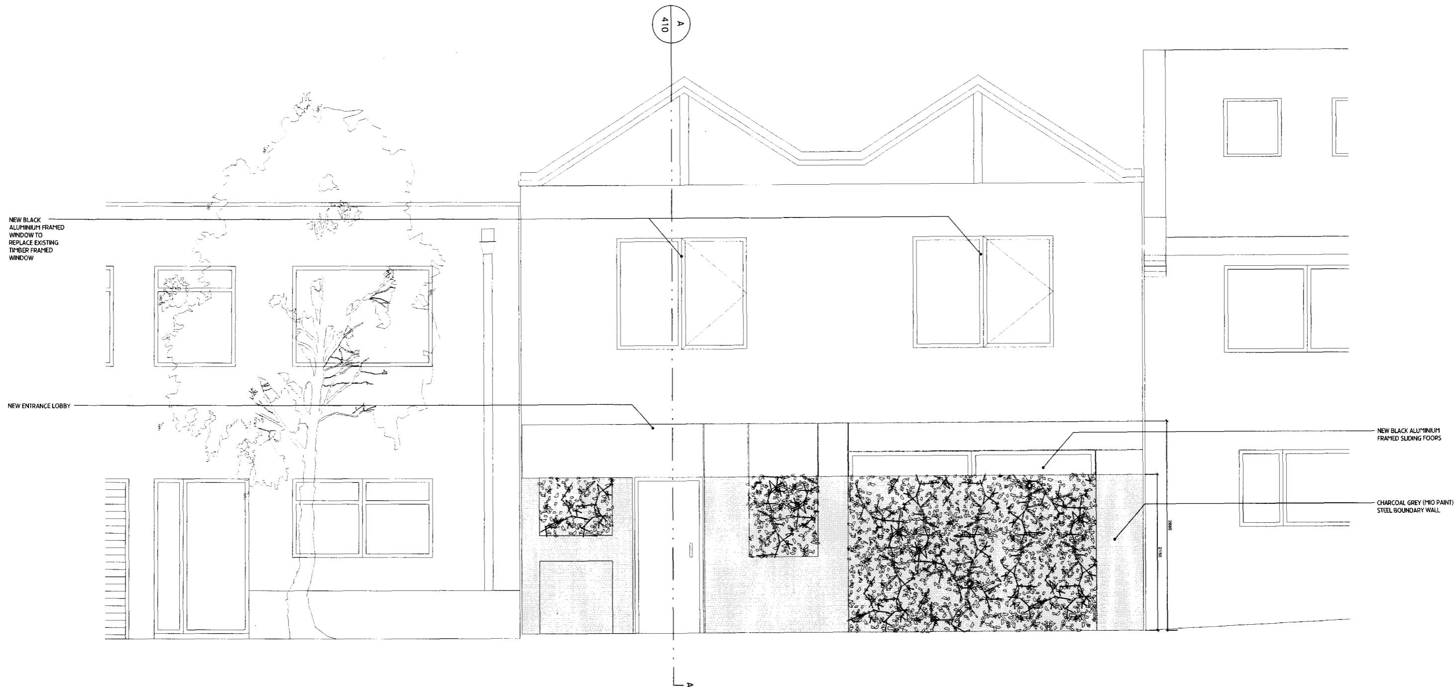
01 PROPOSED FRONT ELEVATION
