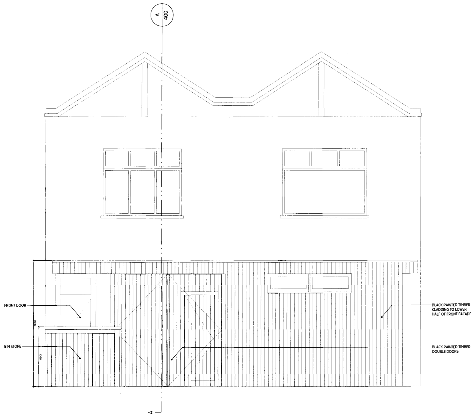
01 EXISTING FRONT ELEVATION
