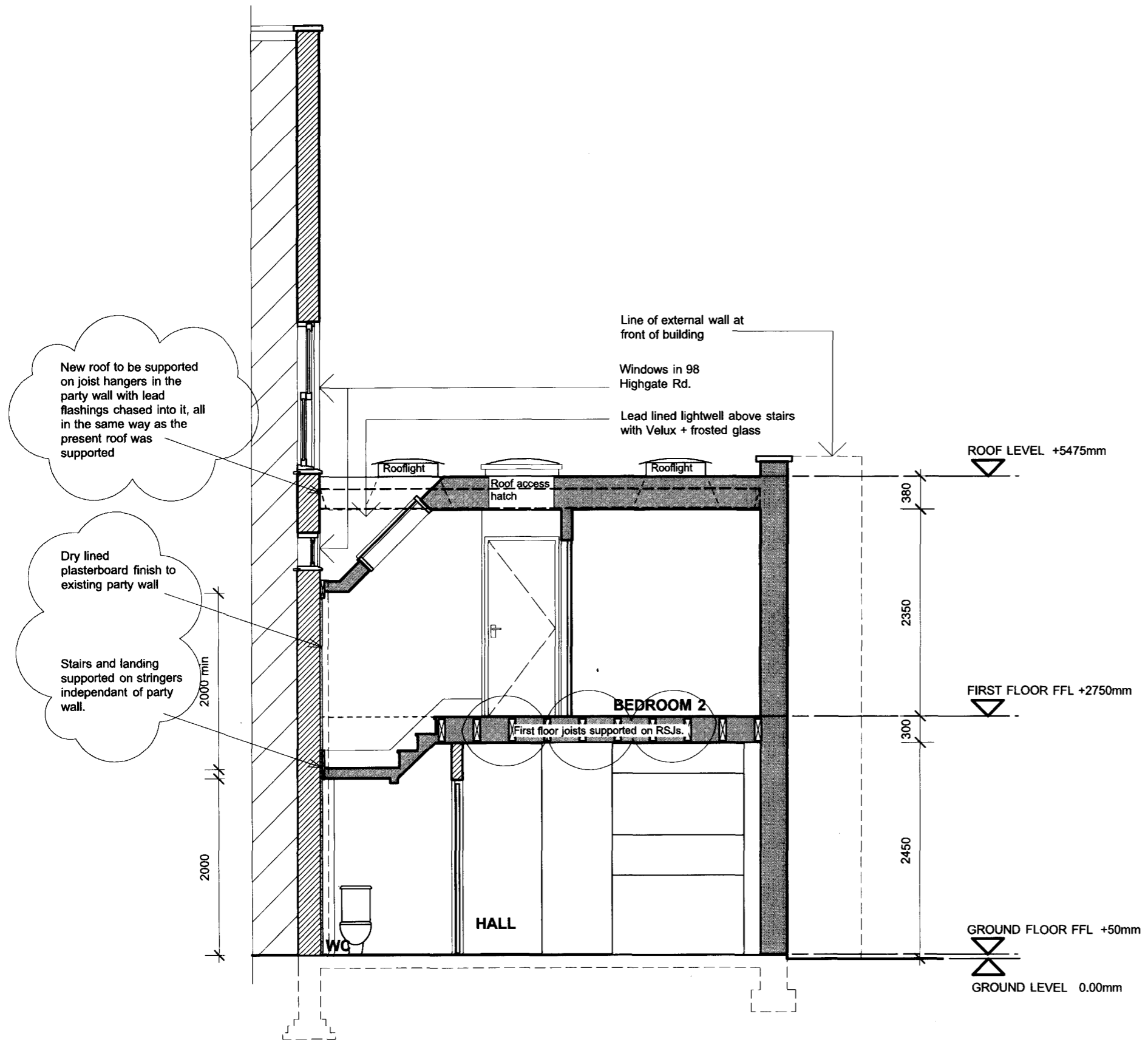
PROPOSED SECTION AA 1:50 @ A3
