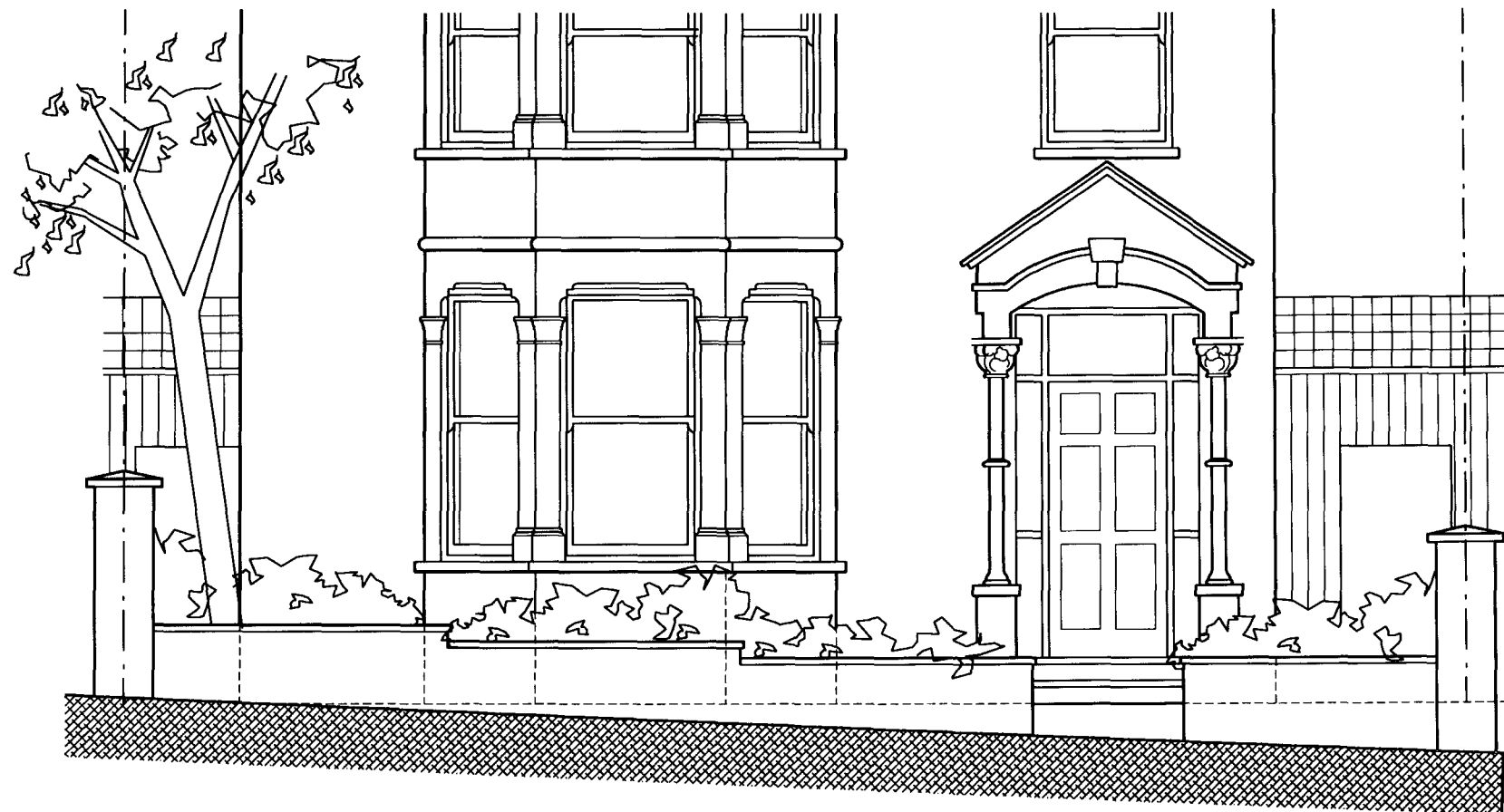
FRONT ELEVATION - in true elevation (AS EXISTING)
