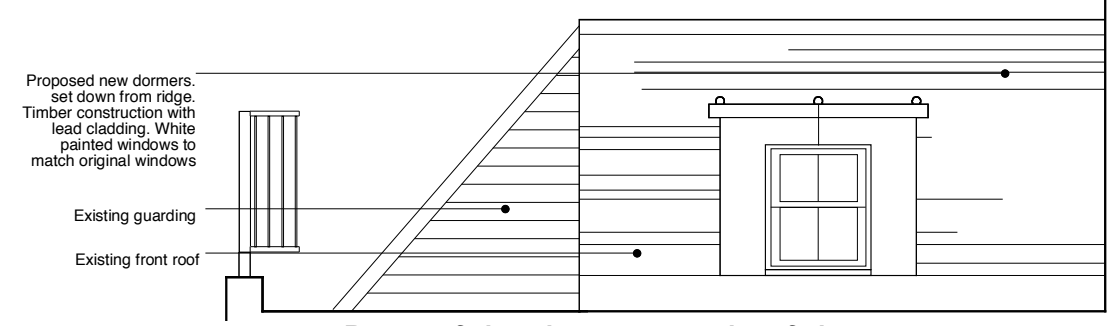
Rear roof elevation on external roof plane
