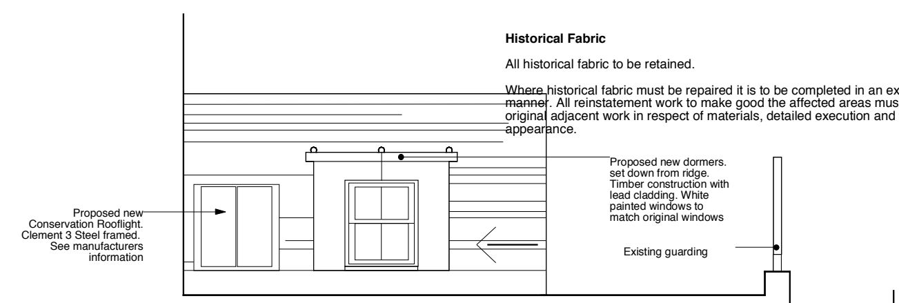
Rear roof elevation between roofs
