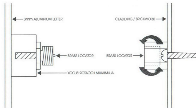
BRASS LOCATOR FIXING DETAIL 1:1 LETTERS AND LOGO PANELS STAND 25mm OFF BUILDING
