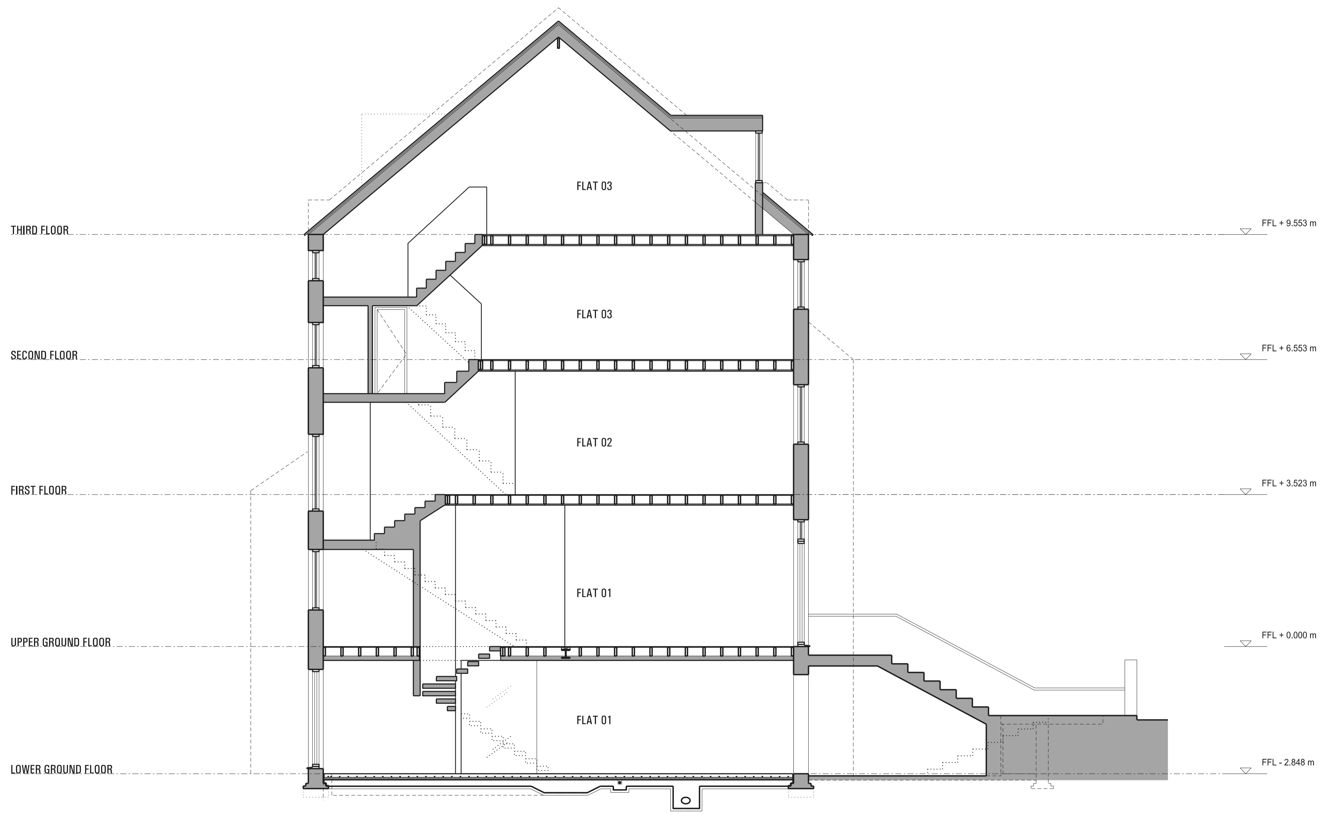
01 SECTION C-C Scale 1:50
