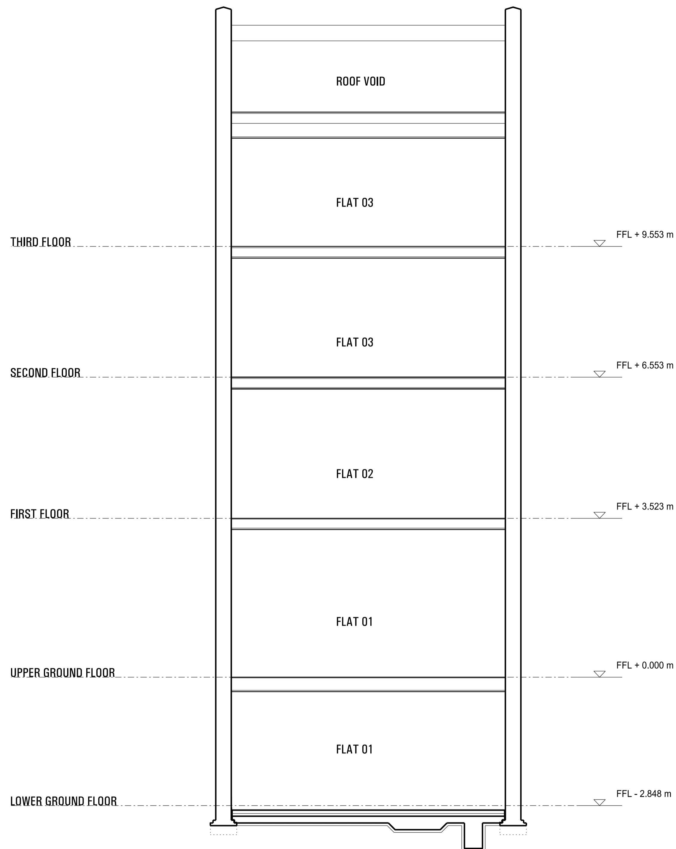
01 SECTION B-B Scale 1:50
