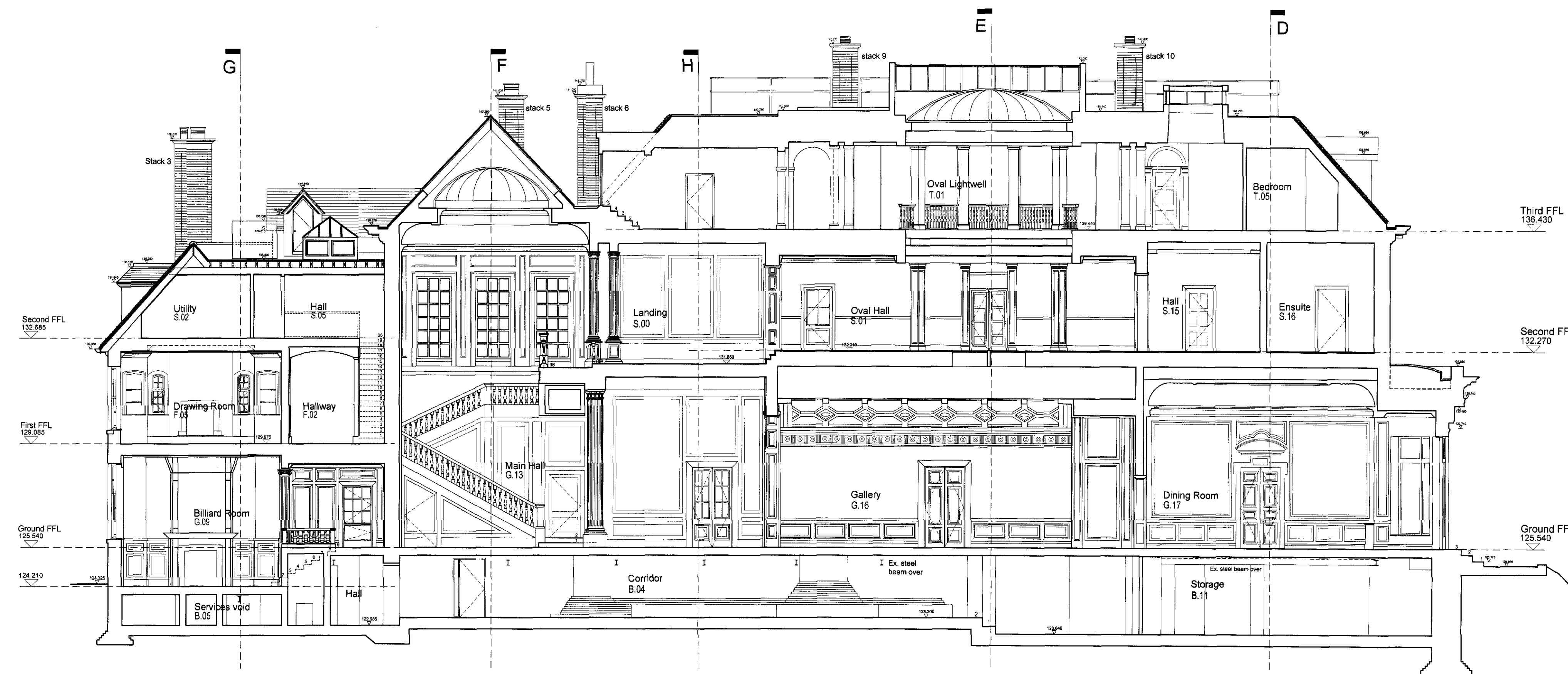
EXISTING SECTION BB. 1:100
