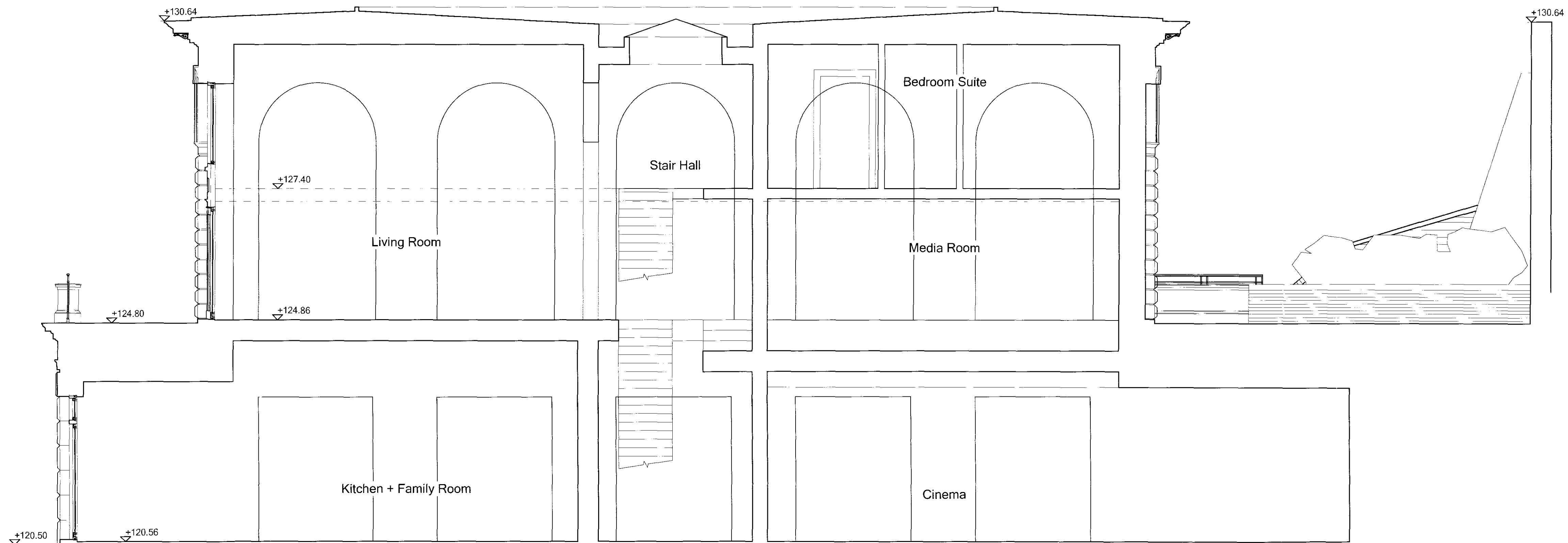
Section L
