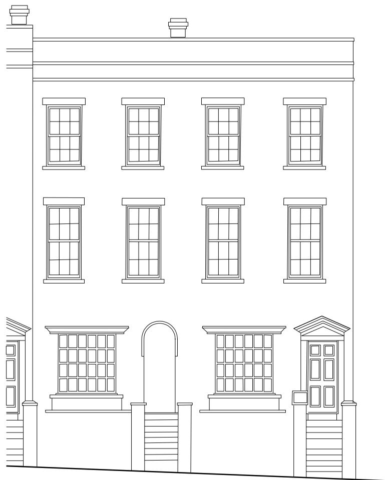
EXISTING FRONT ELEVATION A (FROM FLASK WALK)
