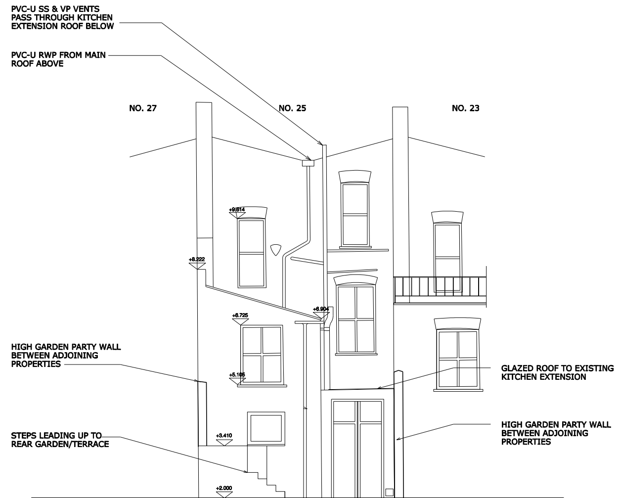
EXISTING REAR ELEVATION B
