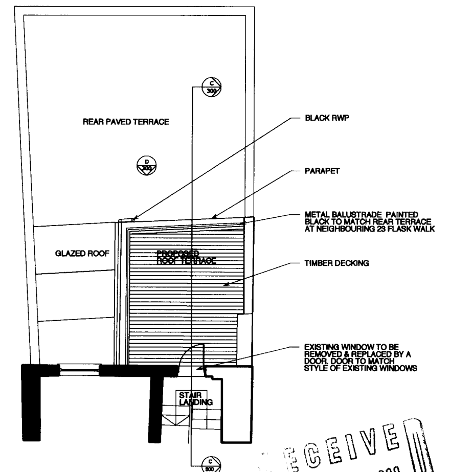
PROPOSED ROOF/PARTIAL 2ND FLOOR PLAN
