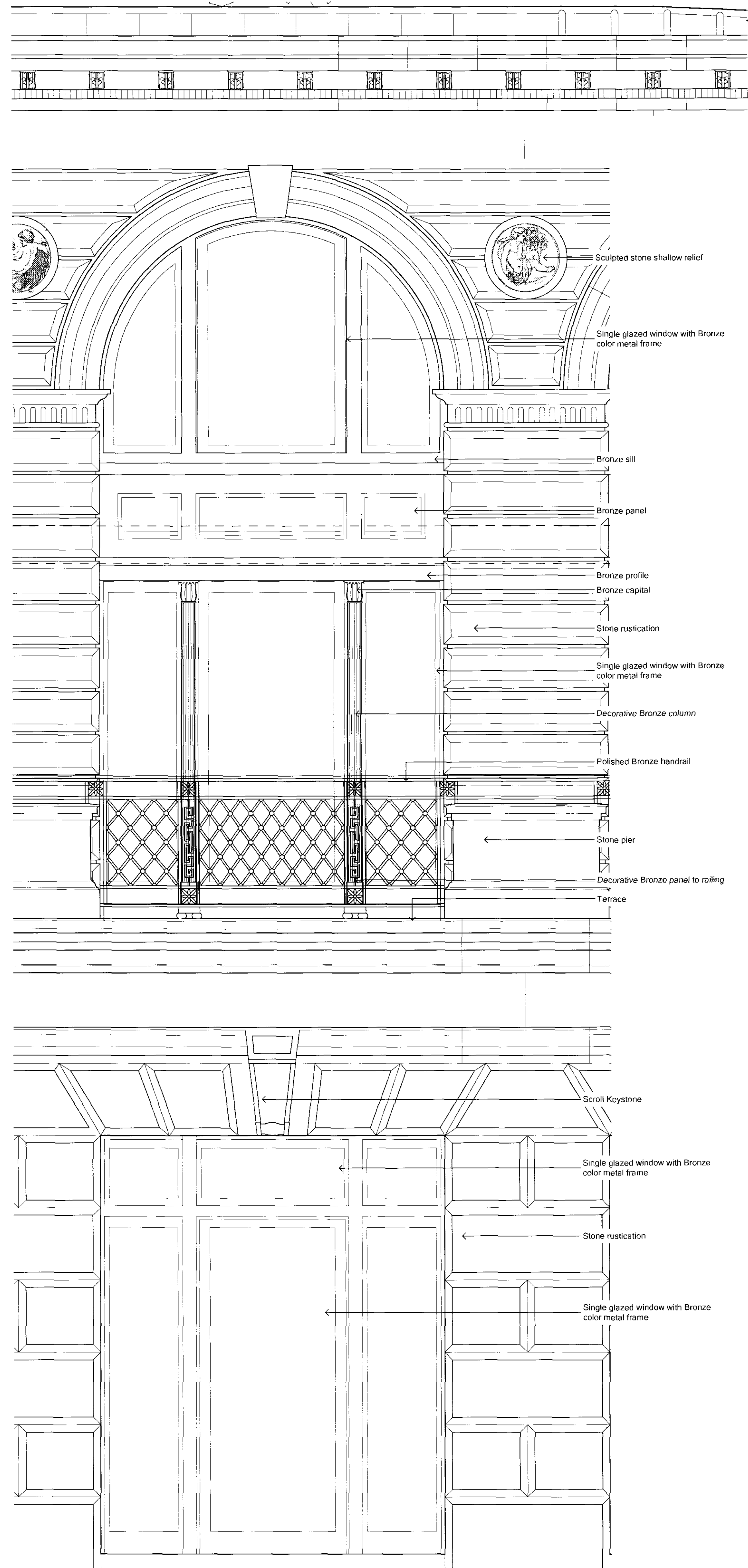
Typical Bay Elevation (Elevation B)
