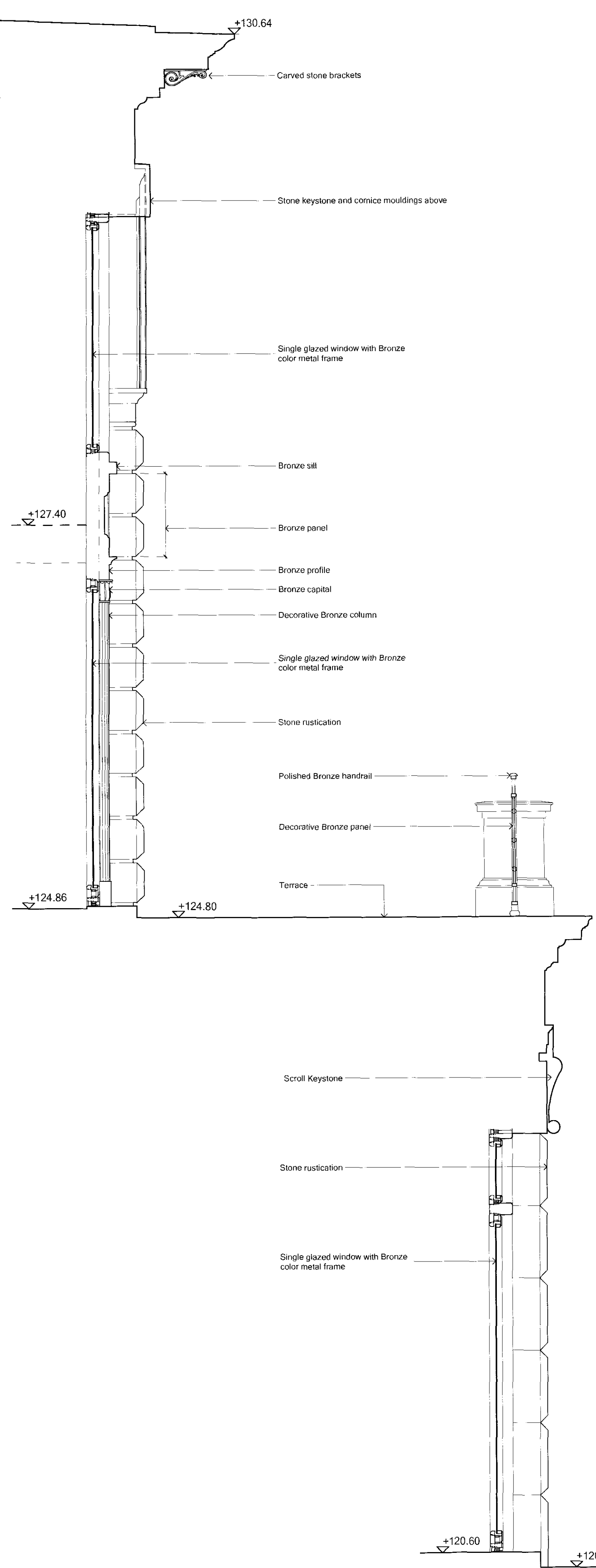
Section through Middle of a Bay (Section A)
