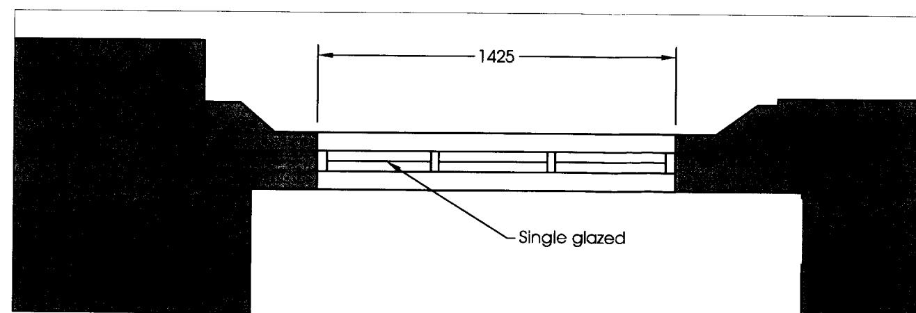
Existing Window Plan (1:20)
