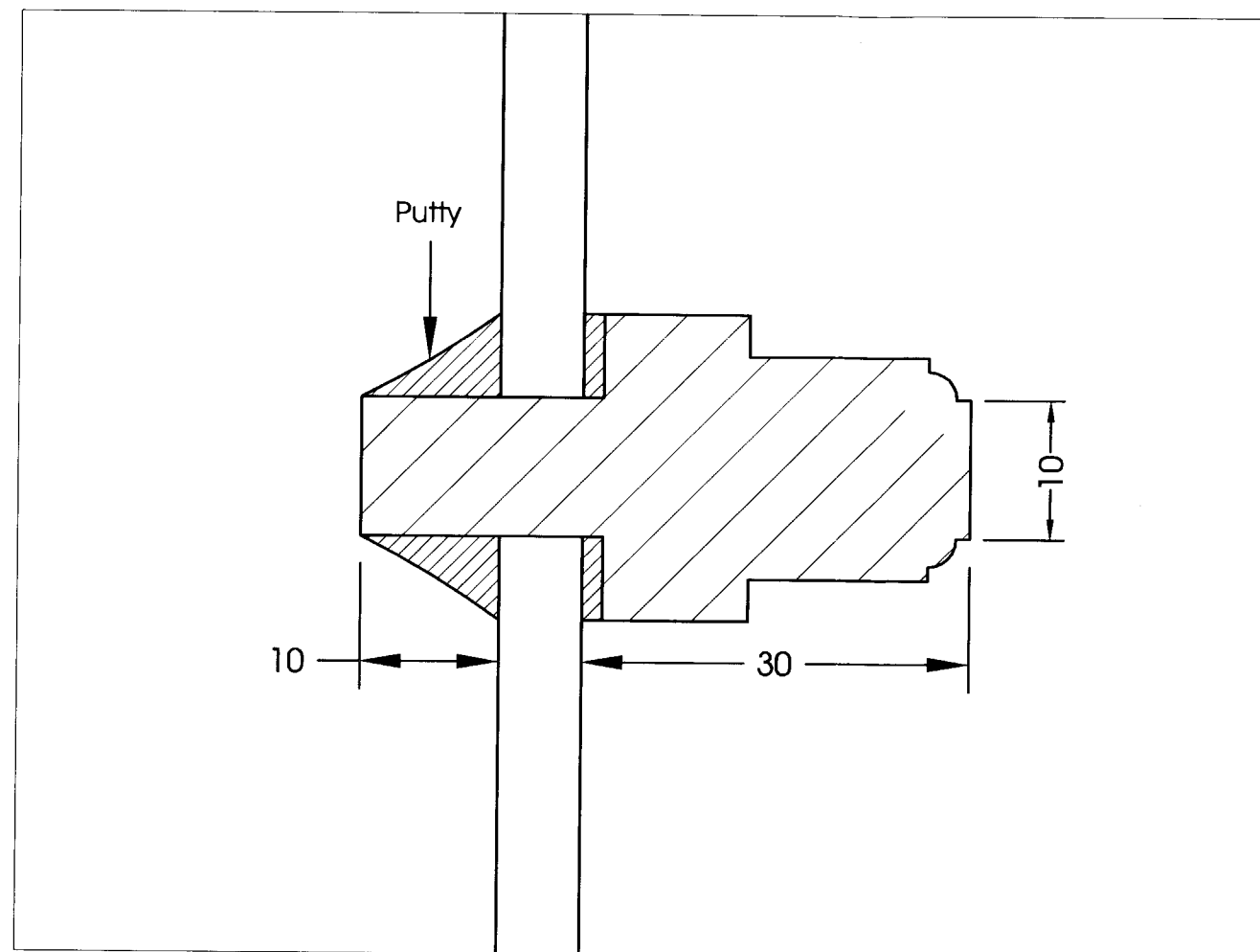
Glazing Bar Detail (2:1)
