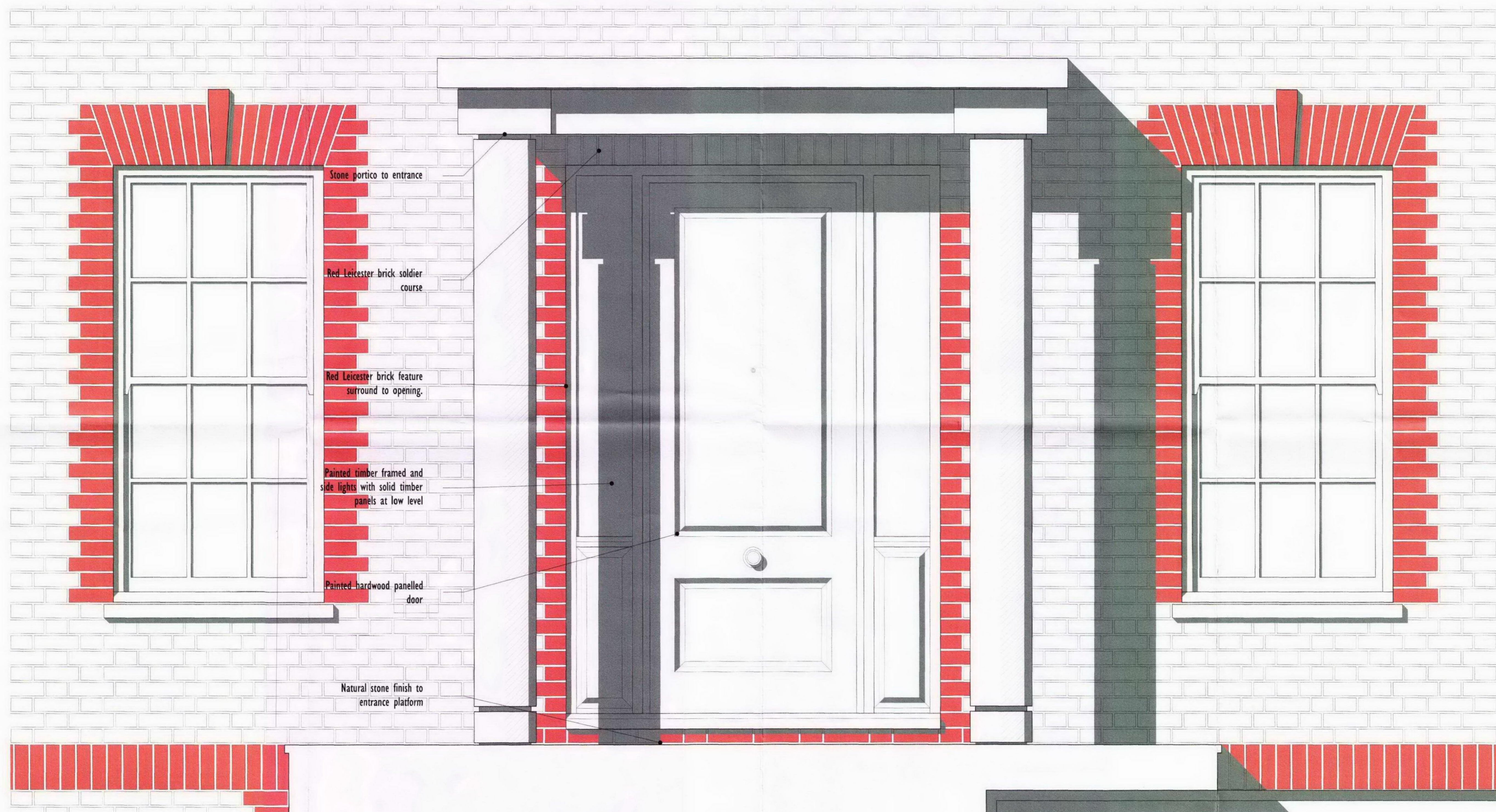
PROPOSED ELEVATION TO QUEEN'S GROVE
