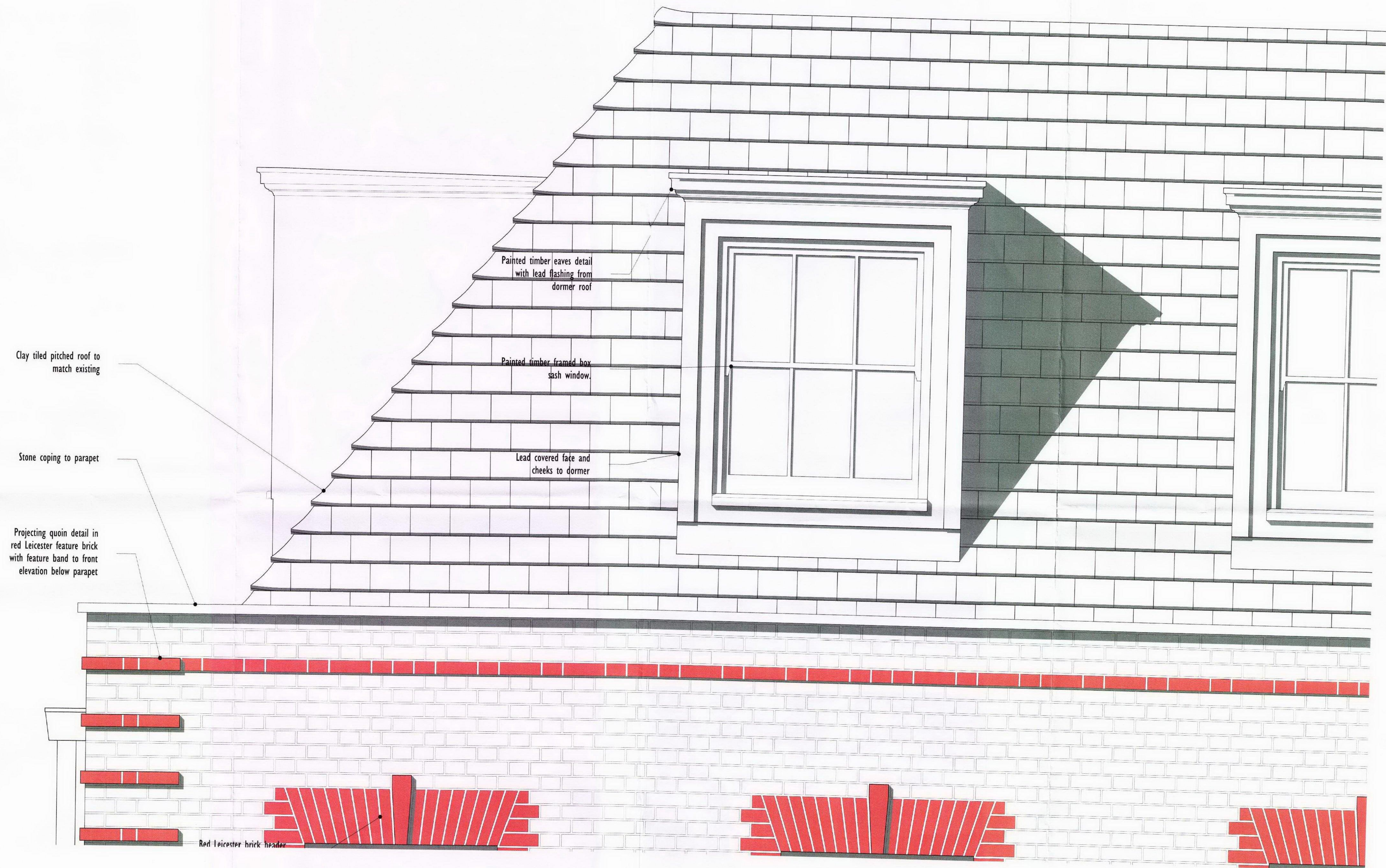
TYPICAL DETAILING TO ROOF, BRICKWORK AND DORMER
