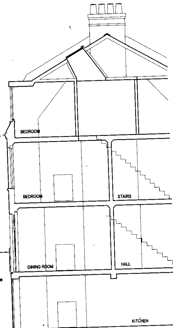
TYPICAL SECTION THRO REAR WALL
