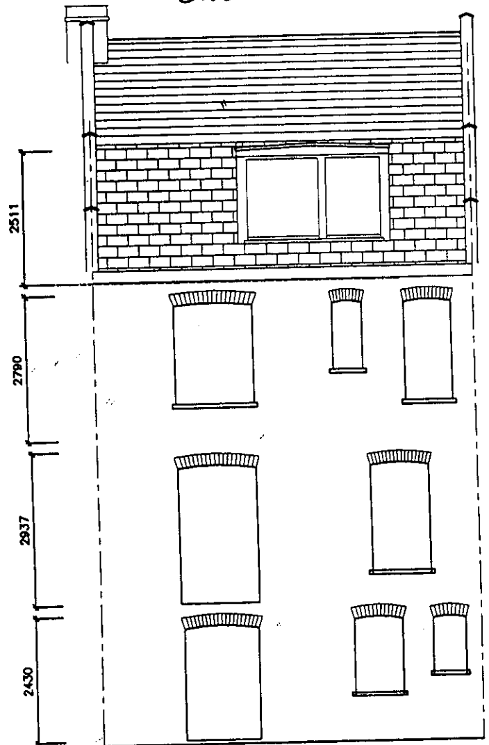
REAR ELEVATION
