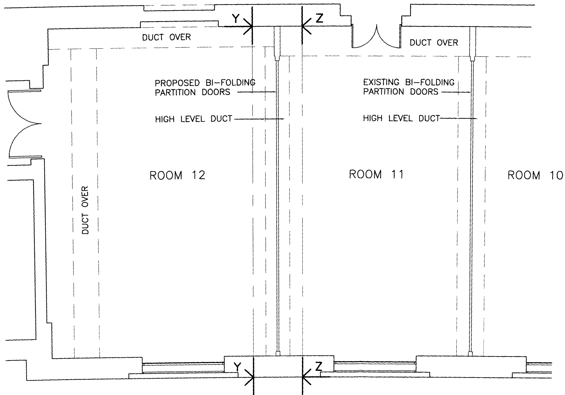
PROPOSED PLAN SCALE 1:50
