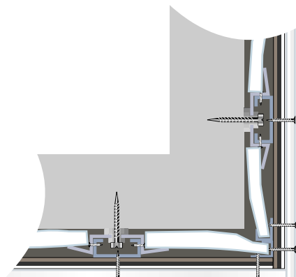
External corner assembly
