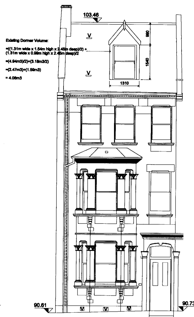
PROPOSED FRONT ELEVATION (NO CHANGE)
