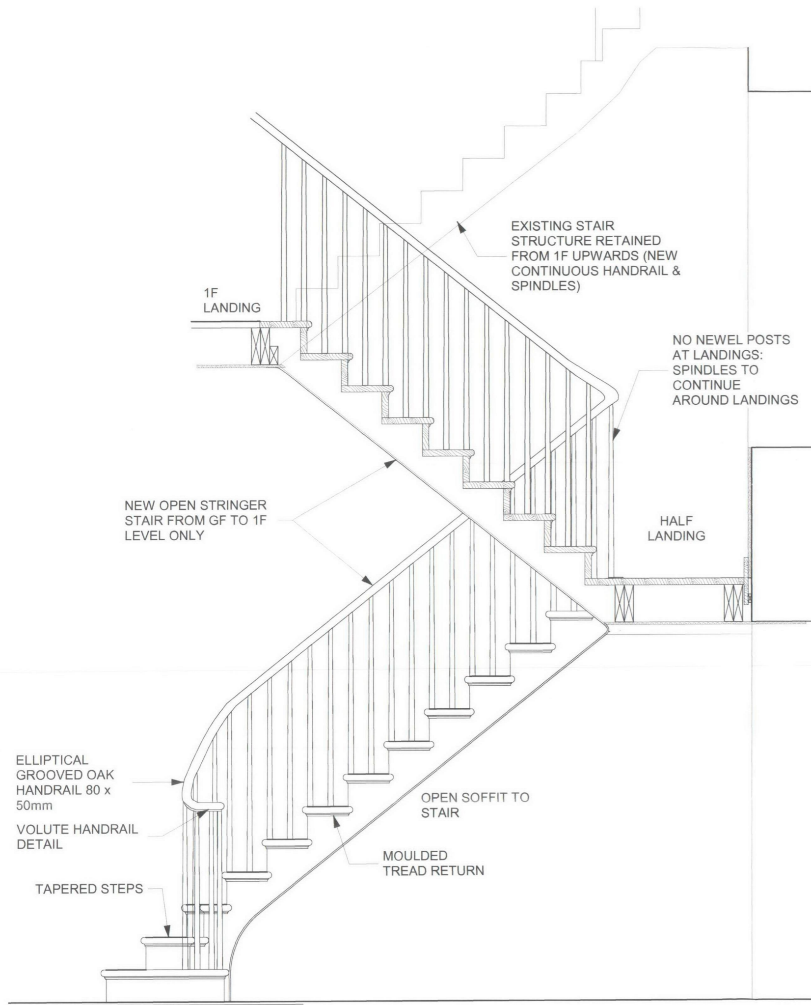
SECTION X-X
