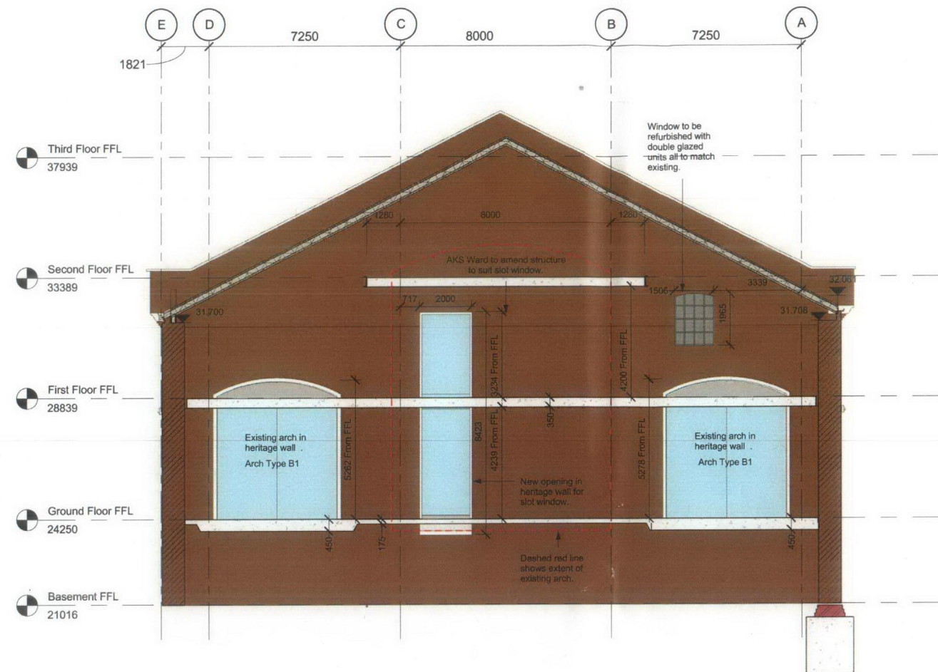
2 ETS HERITAGE WALL INTERIOR NORTH GABLE ELEVATION (PL) 1 : 100
