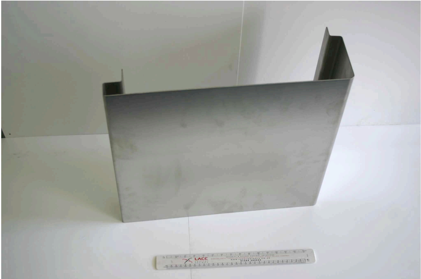
1 Internal portal architrave jamb profile. Profile to LH side opening Upper view showing cross section.
