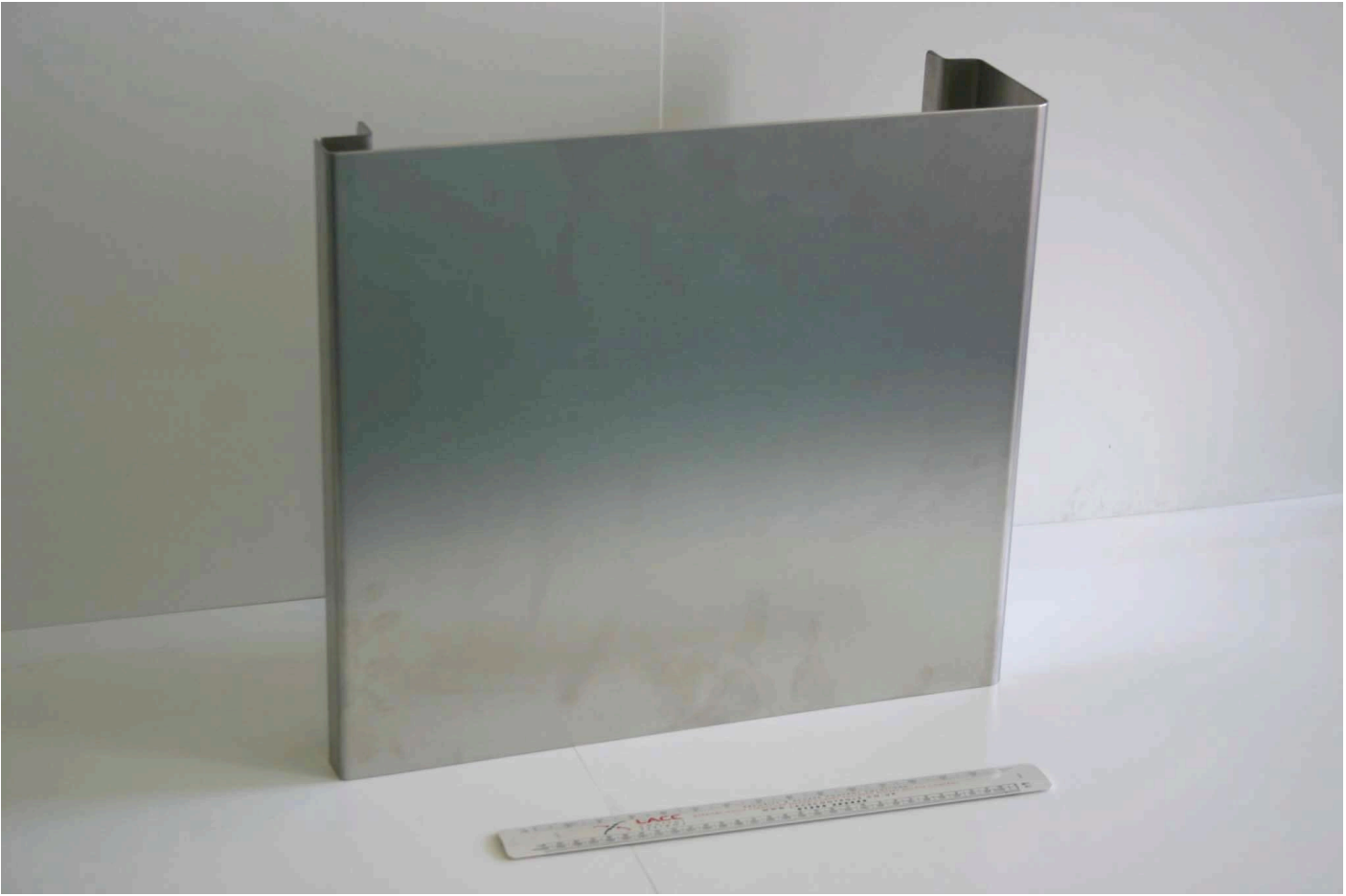
2 Internal portal architrave jamb profile. Profile to LH side opening Face view
