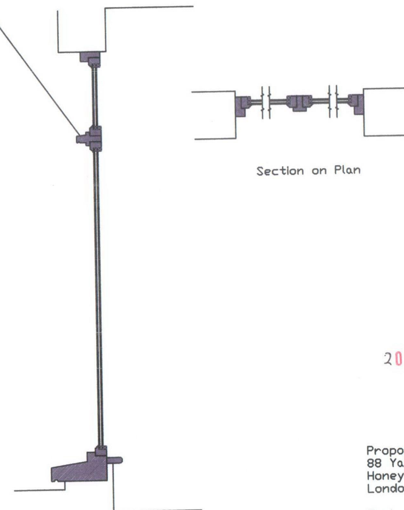
Vertical Section
