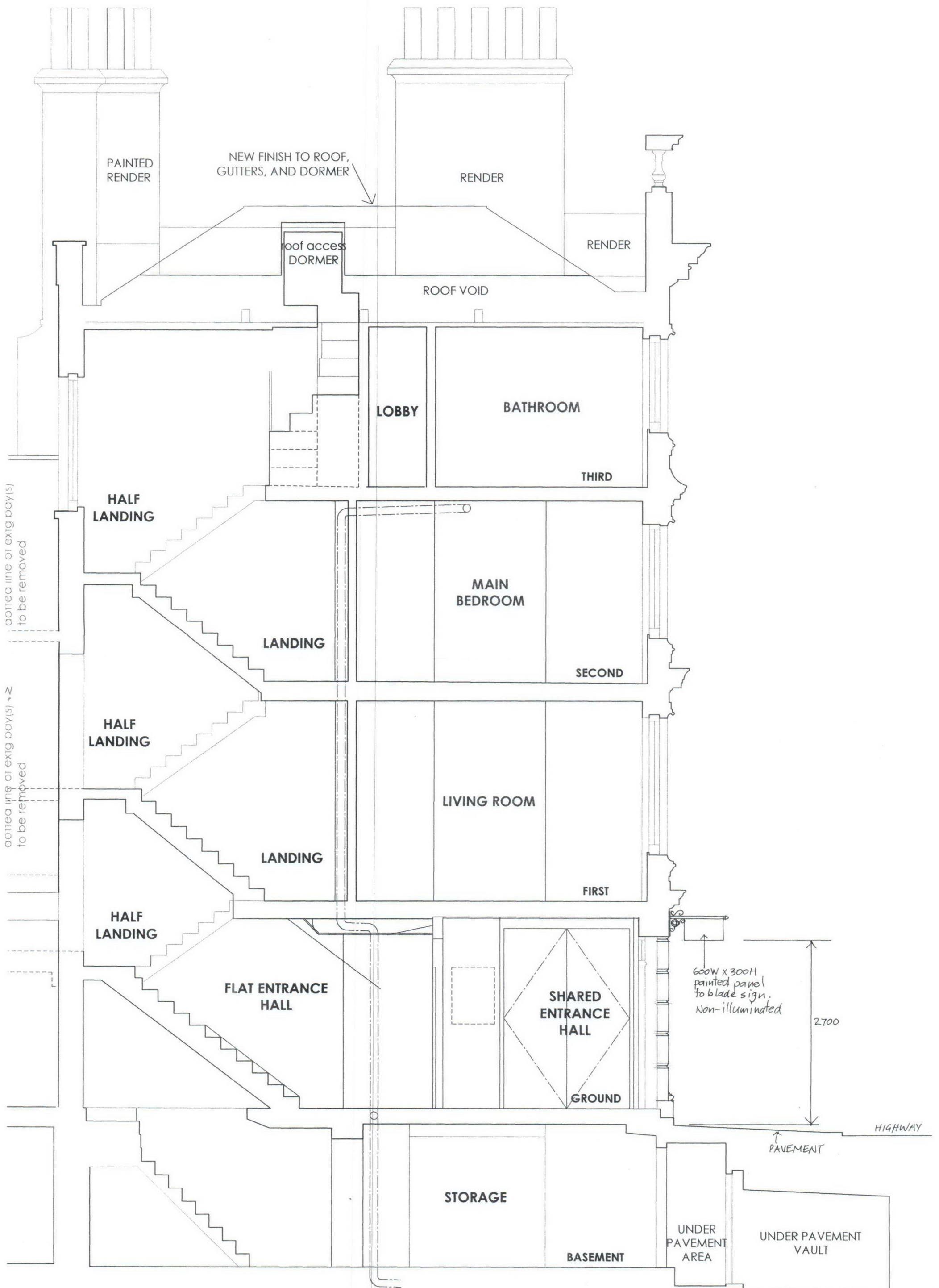
SECTION A-A Showing proposed blade sign 1:50 at A3
