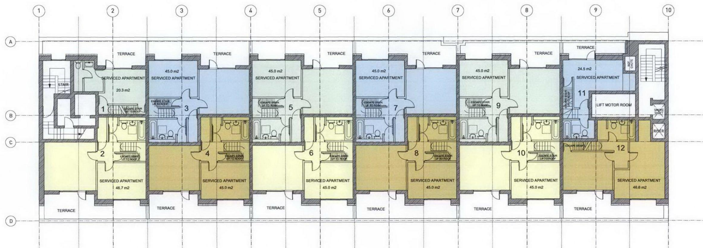
SIXTH FLOOR PLAN AS EXISTING
