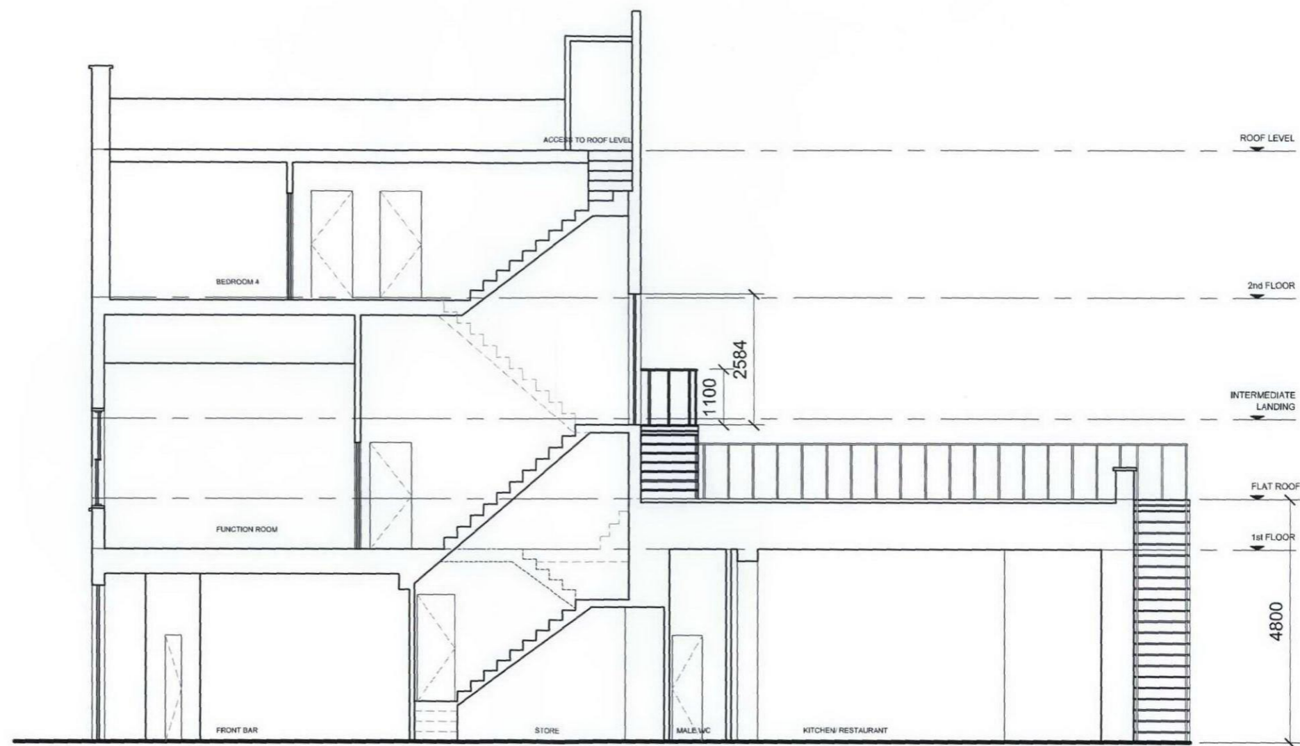
13 PROPOSED SECTION AA 43 Scale: 1:100 @ A3 CAS 10/2009/CAS/Preliminary Floor Plans
