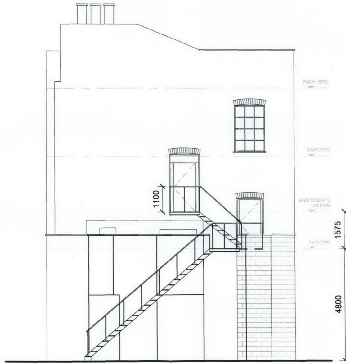
12 PROPOSED REAR ELEVATION 43 Scale: 1:100 @ A3 CAD: R/C/SC/CAB/Preliminary Floor plan
