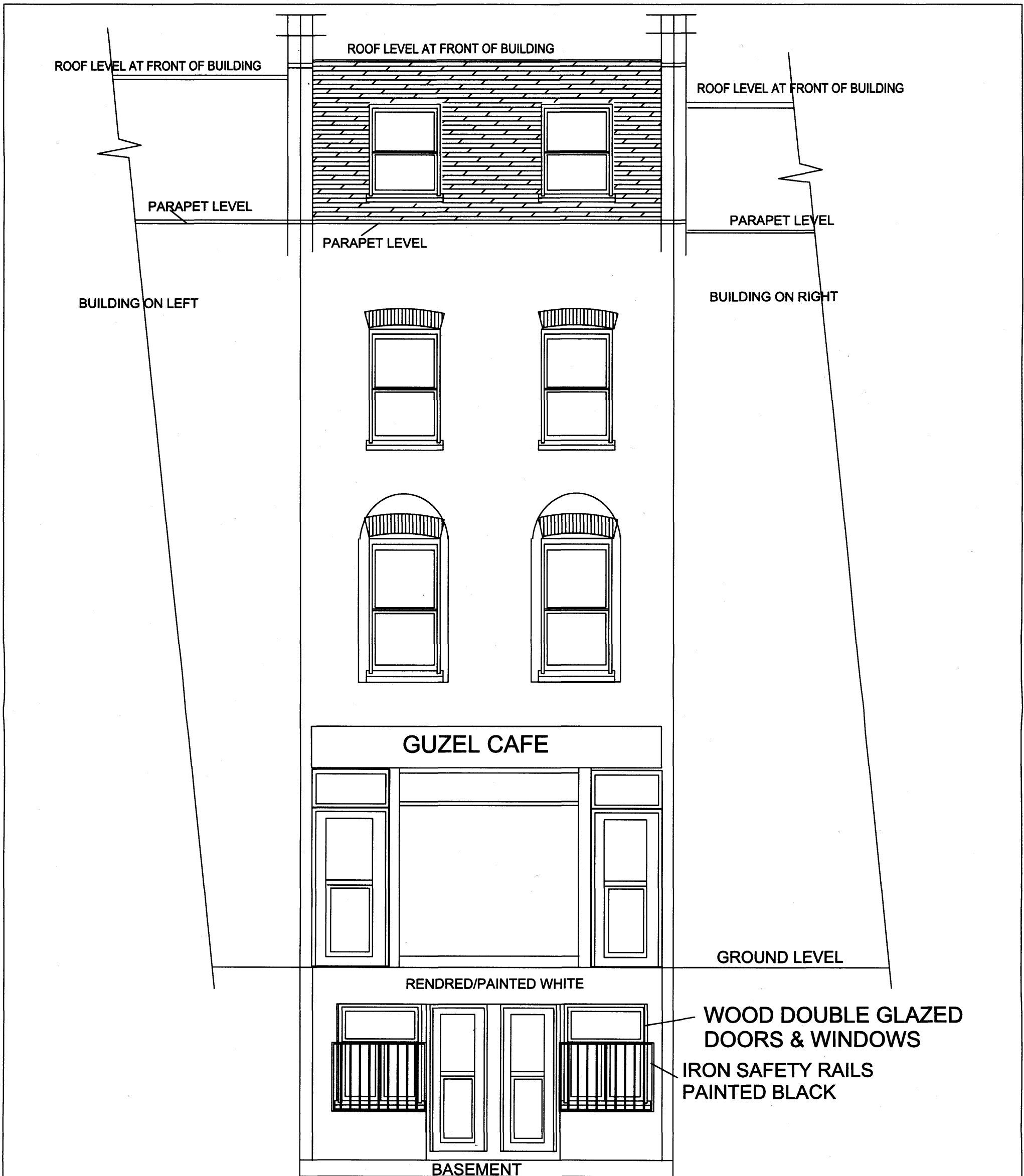
PROPOSED FRONT ELEVATION SECTION VIEW B- B
