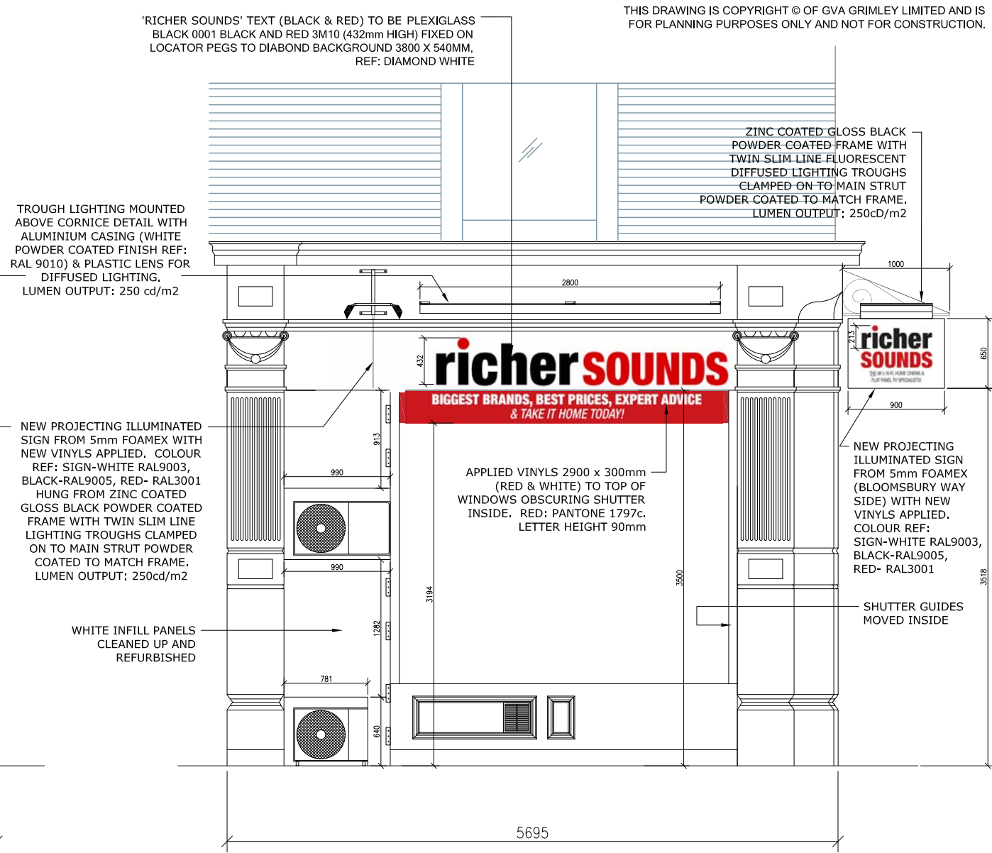
BURY PLACE ELEVATION | 1:50
