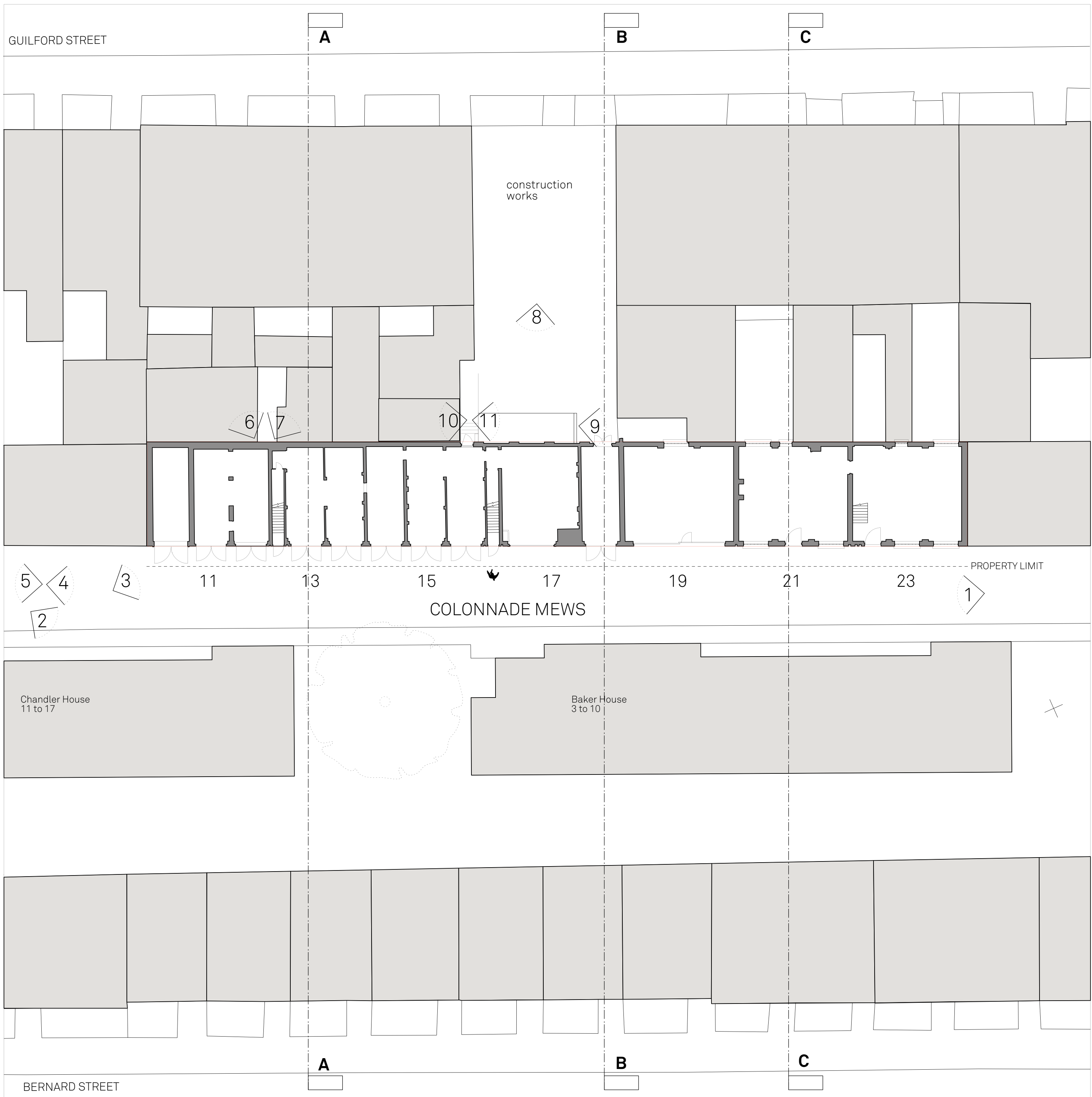
SITE SURVEY PLAN 1:200
