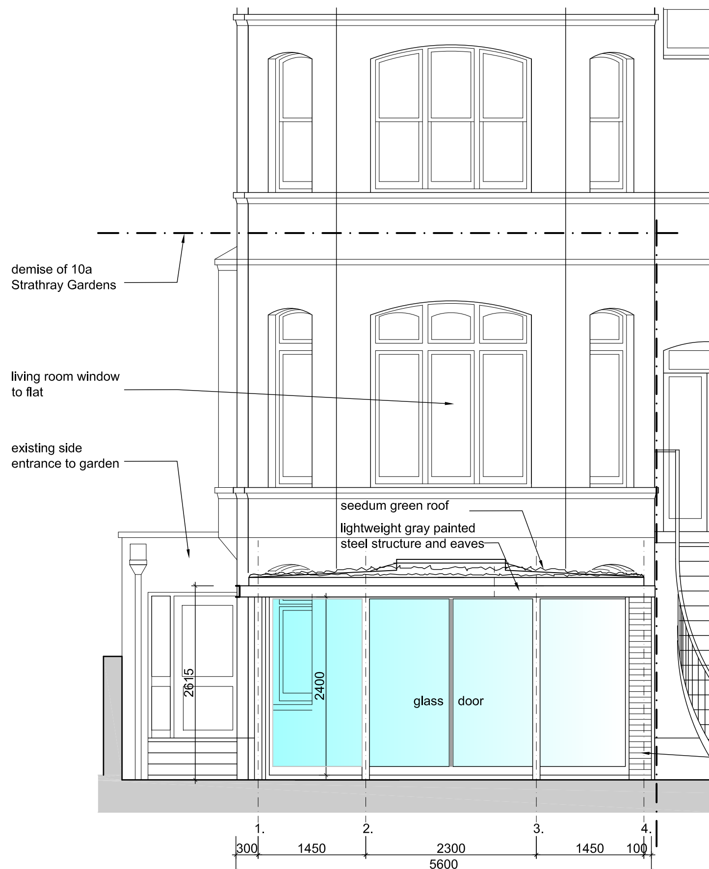
1. Rear (west) Elevation - 1:50
