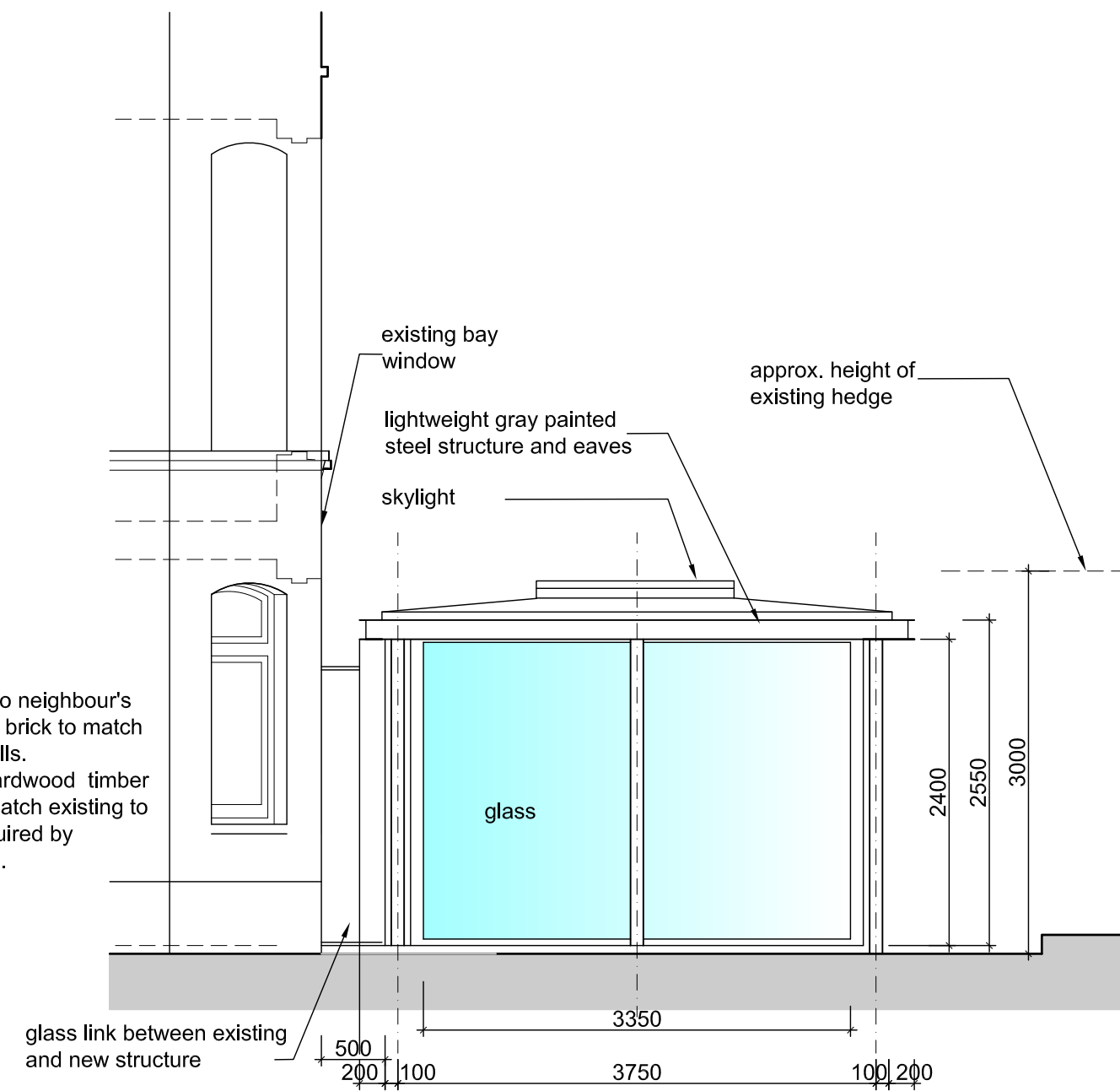
2. Side (north) Elevation - 1:50
