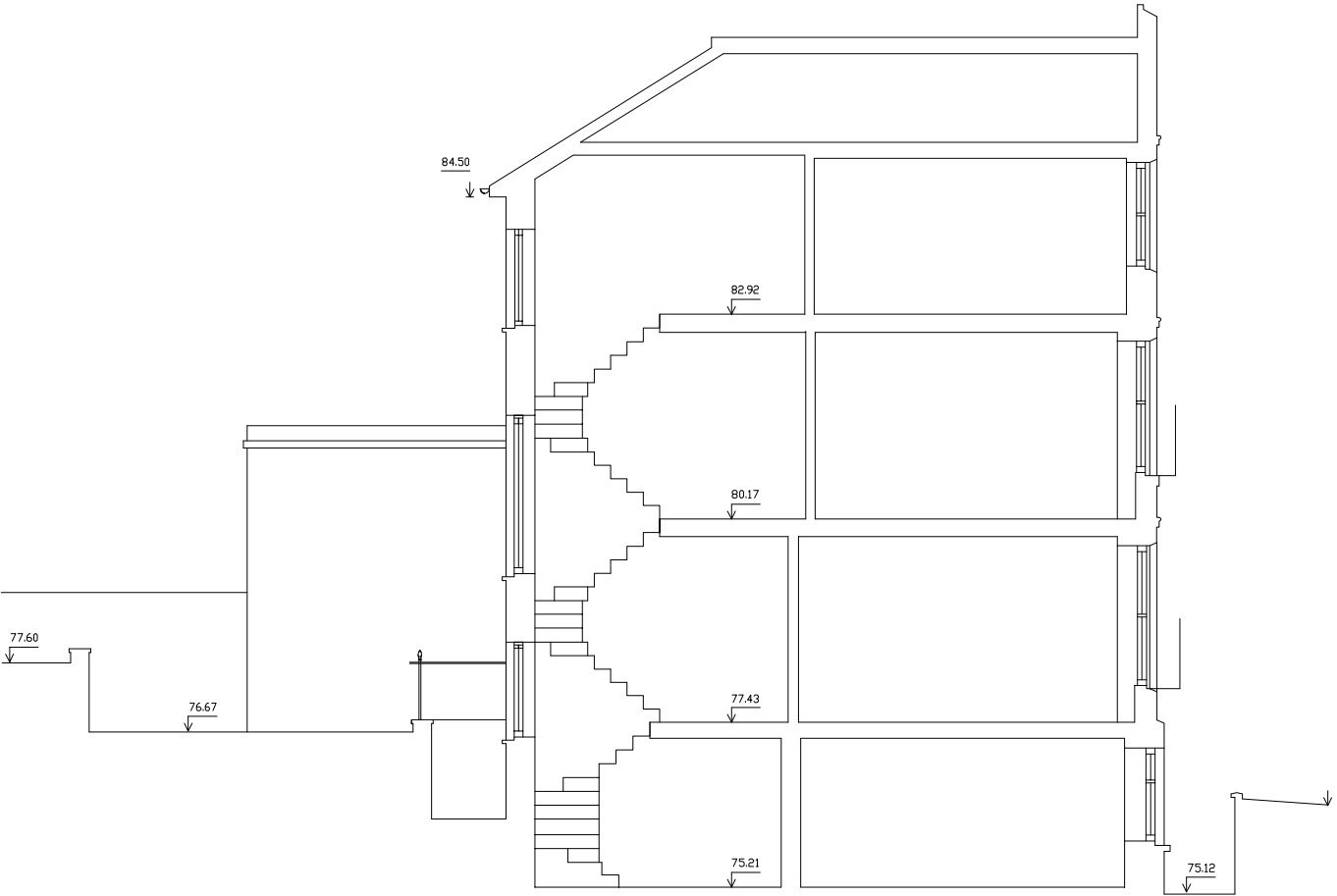
Section AA as existing
