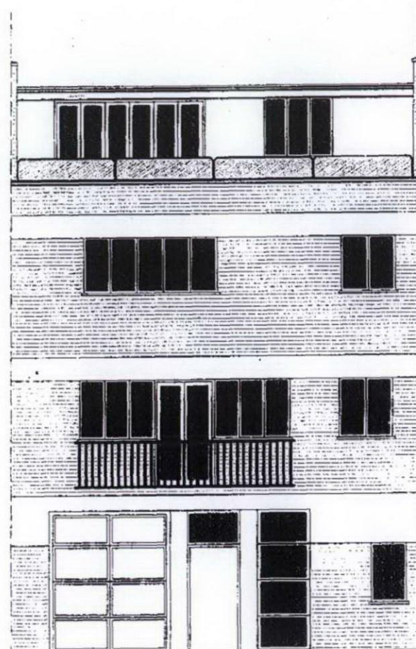
Approved Front Elevation
