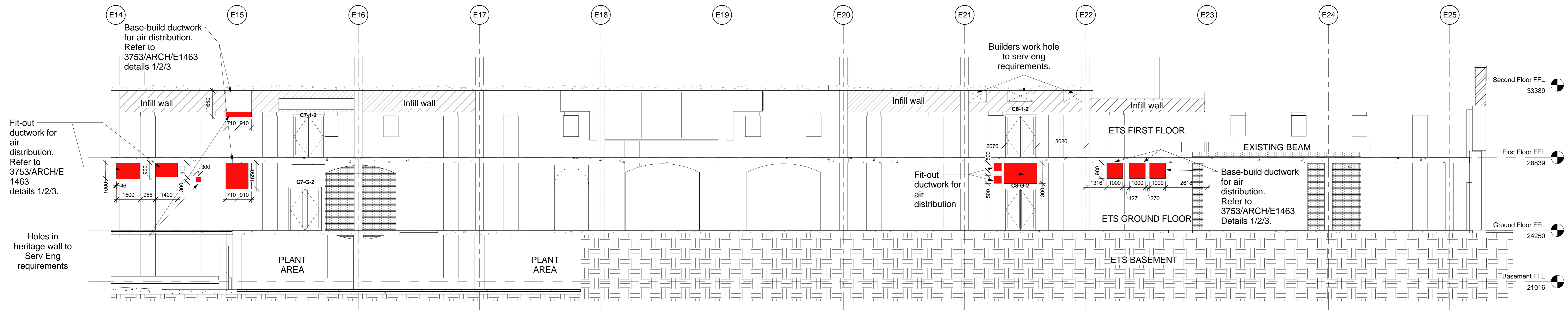
2 Interior Elevation of ETS Gridline D Serv Holes-Planning (cont) 1 : 100
