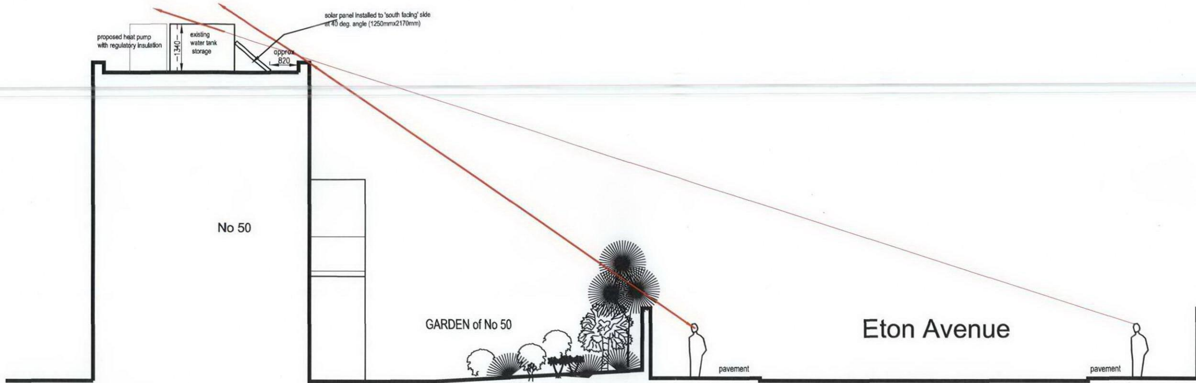
PROPOSED CROSS SECTION X-X SCALE 1:100
