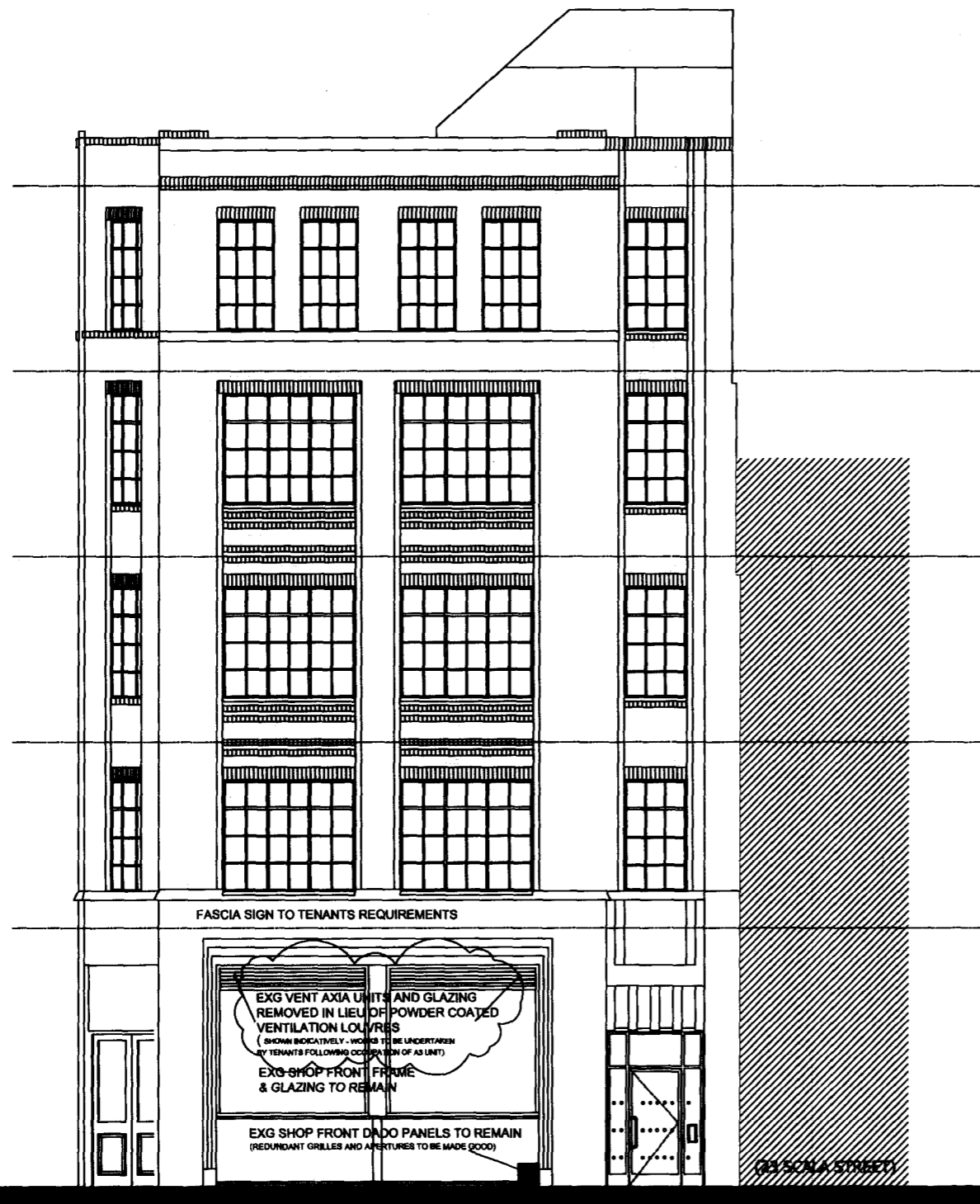
SCALA STREET ELEVATION (NORTH)
