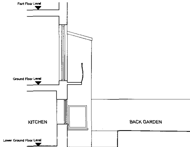
Existing Section A - A (Rear Garden) 1:50
