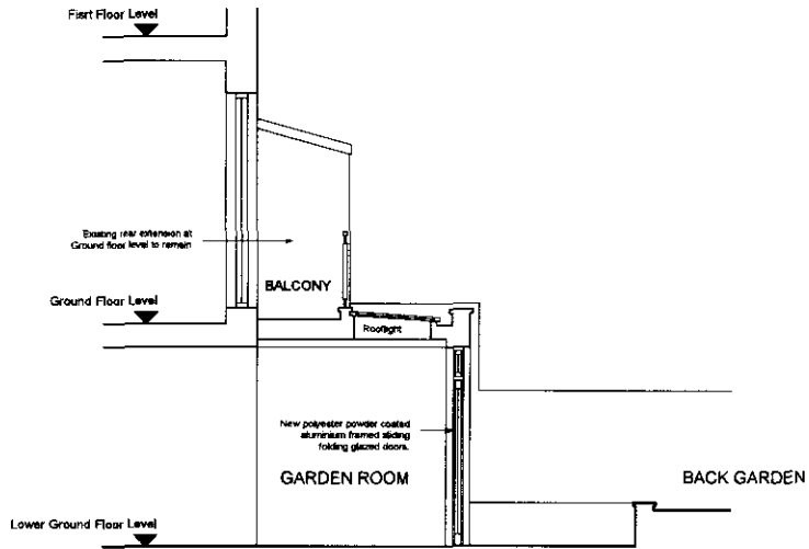
Proposed Section A - A (Rear Extension) 1:50
