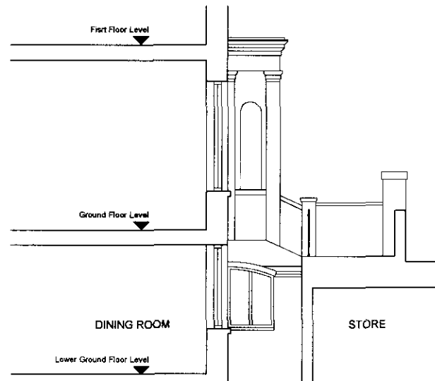
Existing Section B - B (Front Light Well) 1:50
