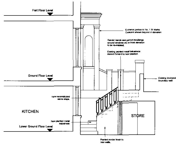
Proposed Section B - B (Front Light Well) 1:50
