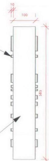
4 PROJECTING SIGN FRONT ELEVATION 304 1:10
