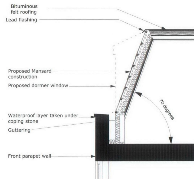
Mansard Section Detail (1:50@A3)
