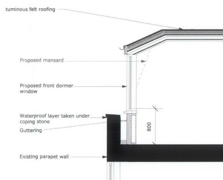
Dormer Window Section Detail (1:50@A3)
