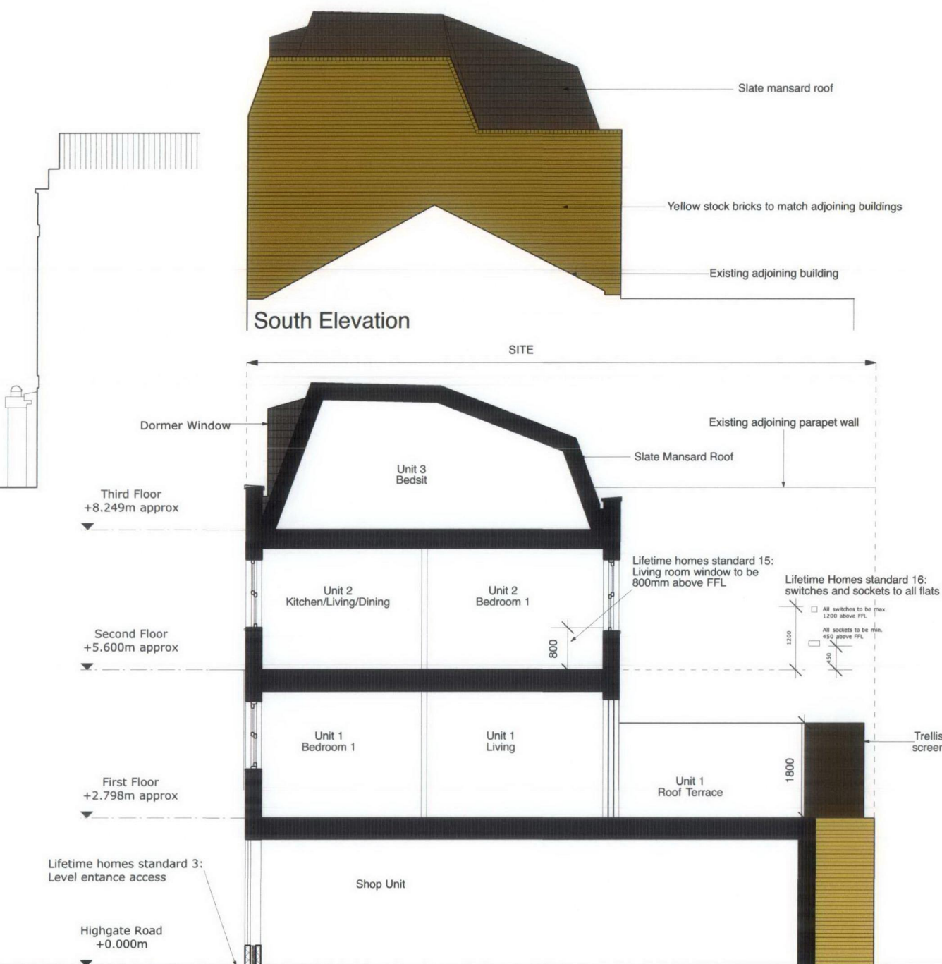
Long Section
