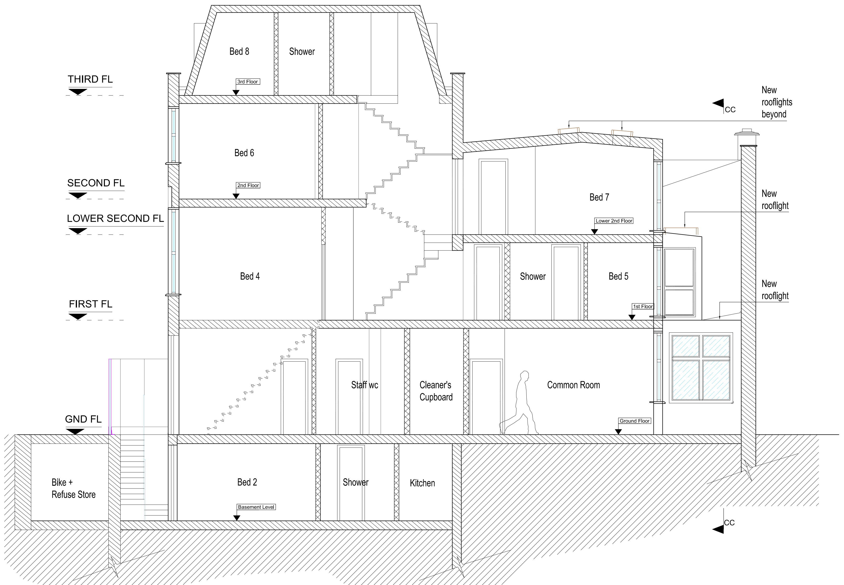
Proposed Section B-B
