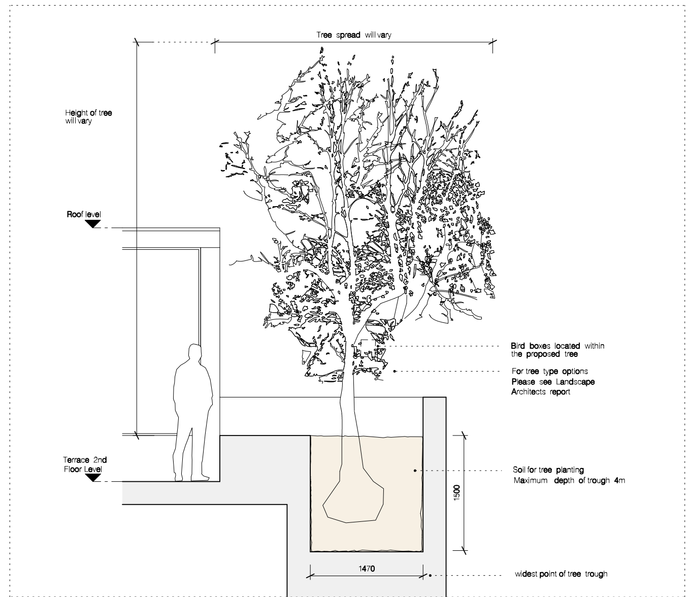
2 Section A of proposed tree at 2nd Floor Level 138 1:50
