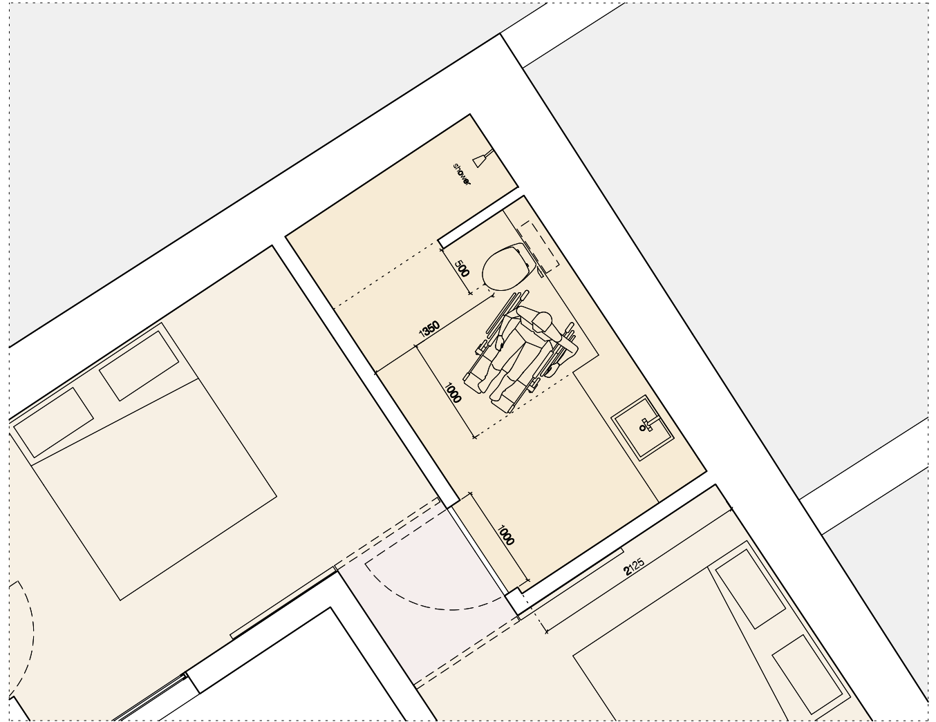
2 136 Plan of Disabled WC at Entrance Level 1:50
