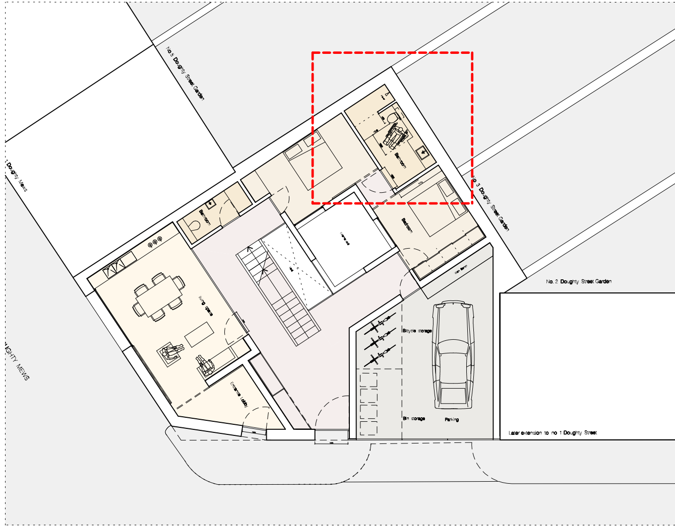
1 136 Location Plan of Disabled WC at Entrance Level
