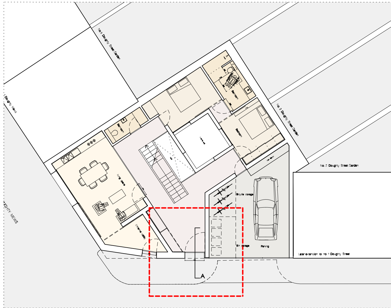
1 134 Location Plan of Entrance Threshold
