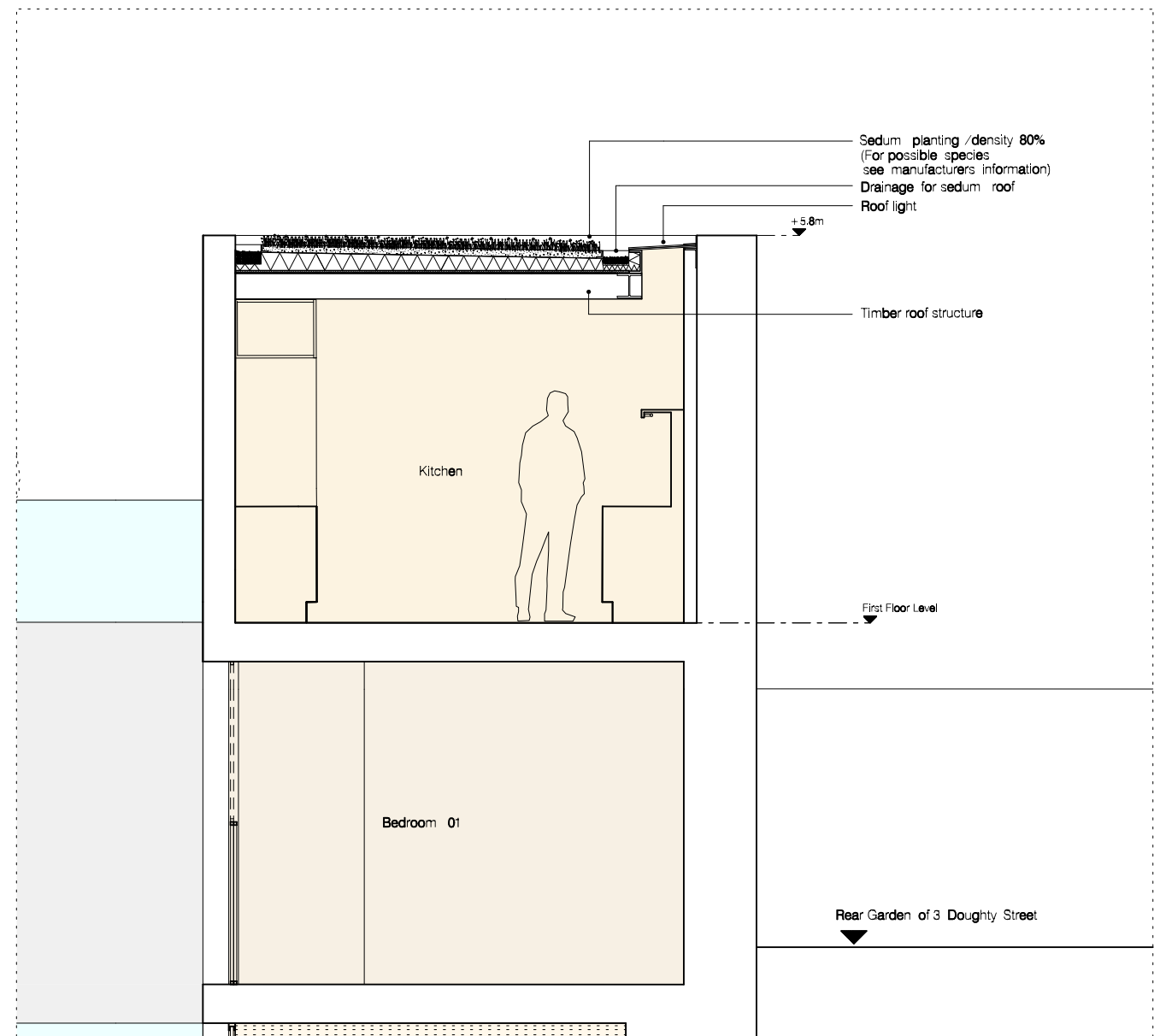
2 139 Section C Green Roof 1:50
