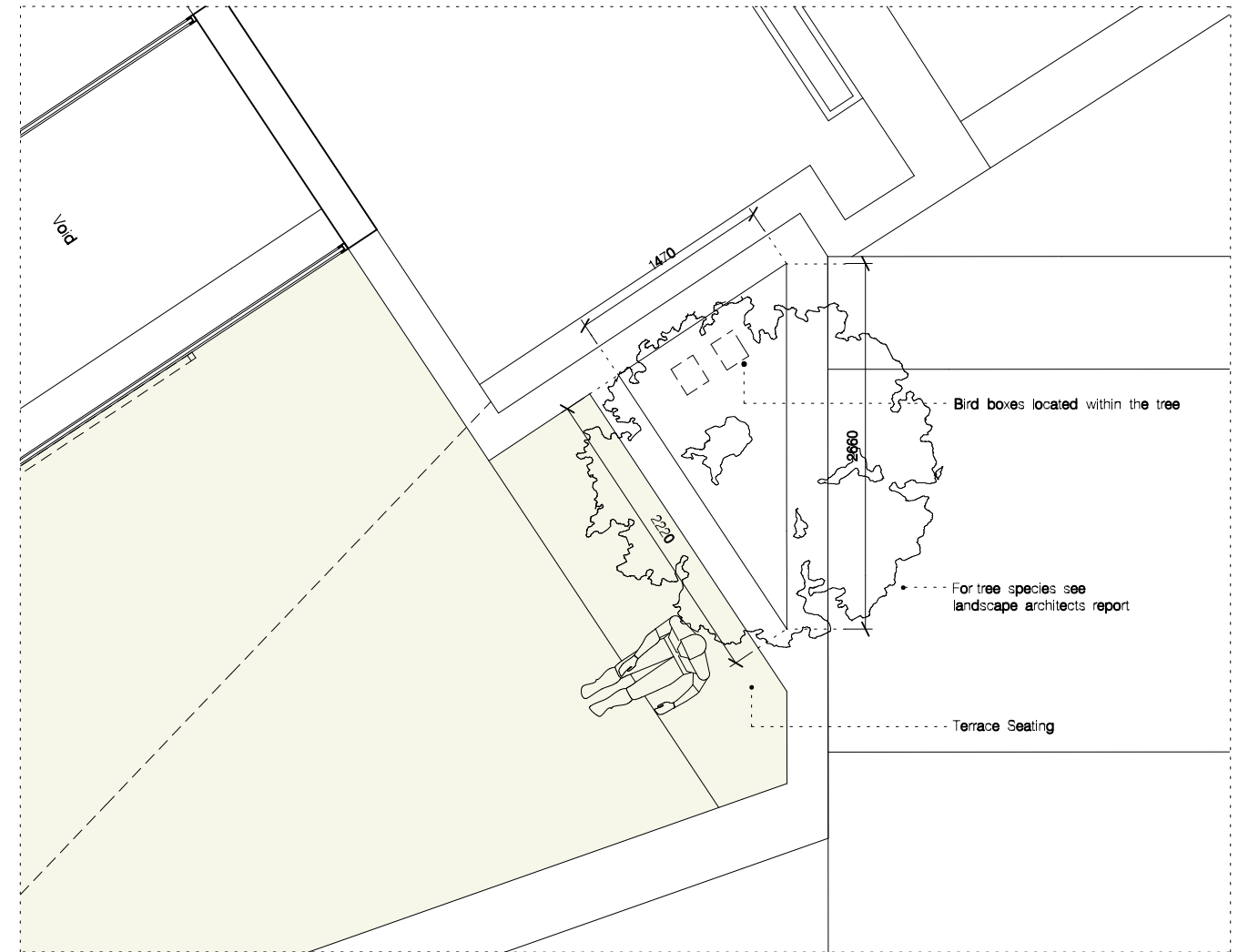
2 Plan of proposed tree at 2nd Floor Level 137 1:50
