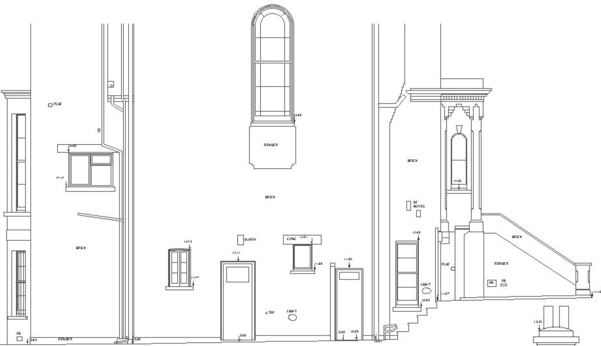
EAST ELEVATION
