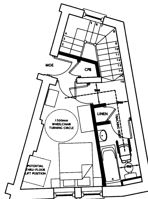
UPPER FLOOR 1:100
