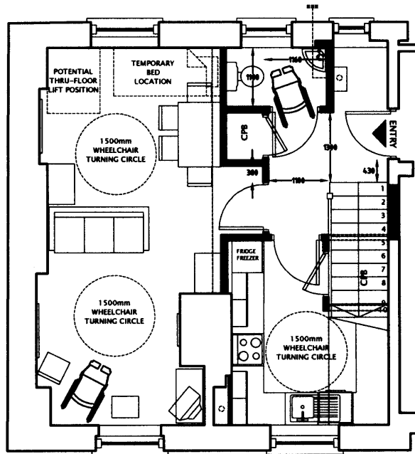
LOWER FLOOR PLAN 1:100
