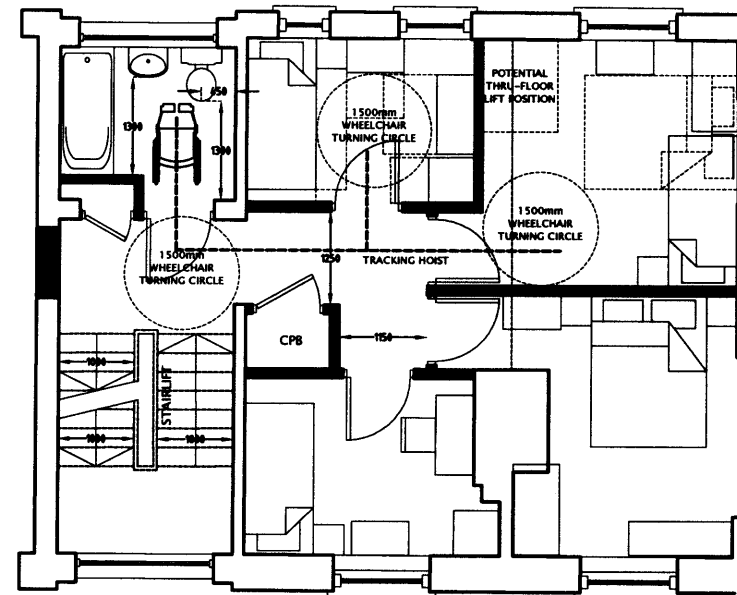
LOWER FLOOR PLAN 1:100
