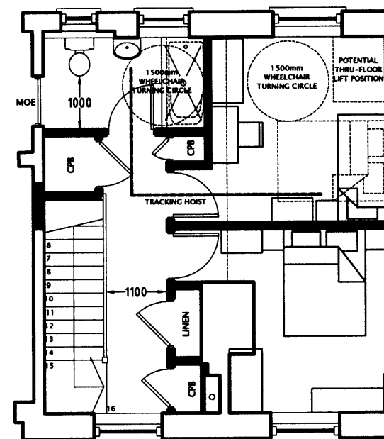
UPPER FLOOR PLAN 1:100
