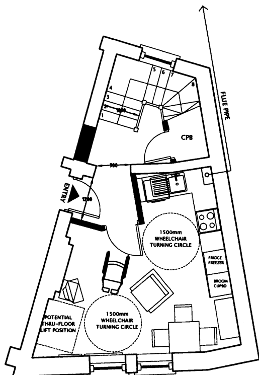
LOWER FLOOR 1:100
