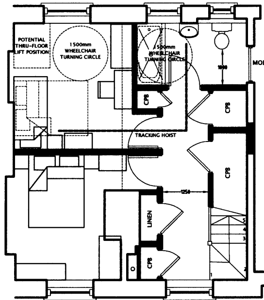
LOWER FLOOR PLAN 1:100
