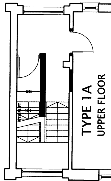
ENTRANCE 1:100
