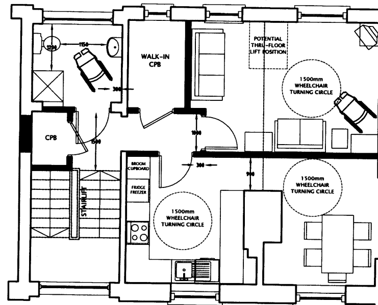
UPPER FLOOR PLAN 1:100
